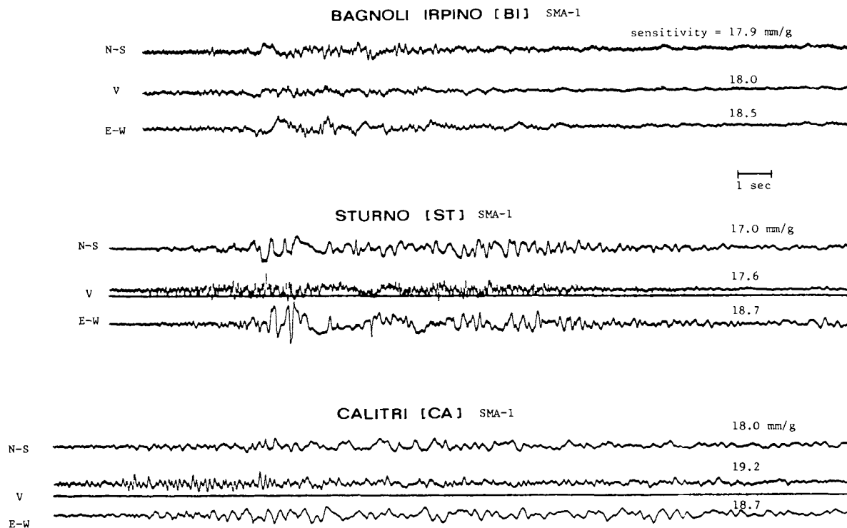
Fig. 4. Strong-motion accelerograms obtained at the stations closest to the source (sensitivities refer to the trace amplitudes in their original size on the 70 mm film records).
