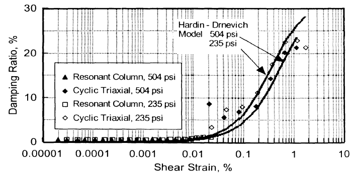
Figure 2. Damping Ratio versus Shear Strain for Ottawa Sand
