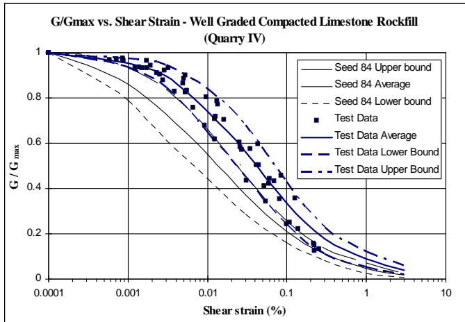
Fig. 9: Variation of G/G_{max} with shear strain – well graded compacted limestone rockfill
