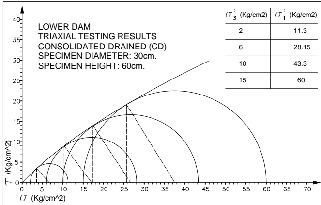
Fig. 3: Mohr-Coulomb Diagram of modeled rockfill
