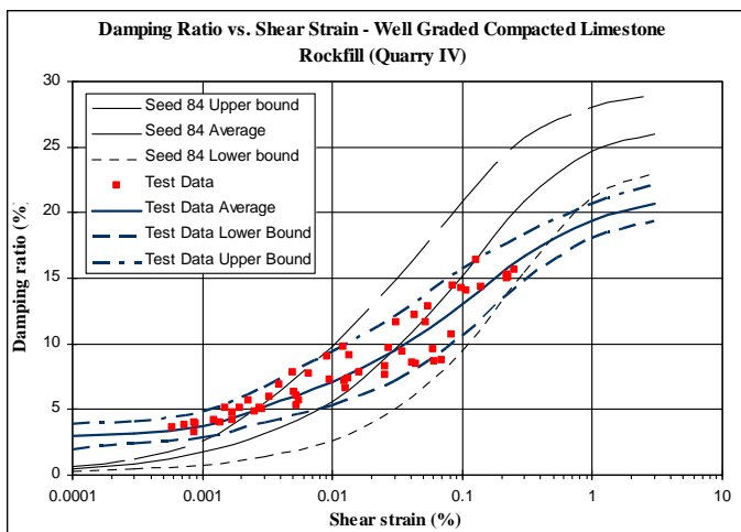
Fig. 10: Variation of damping ratio with shear strain–well graded compacted limestone rockfill
