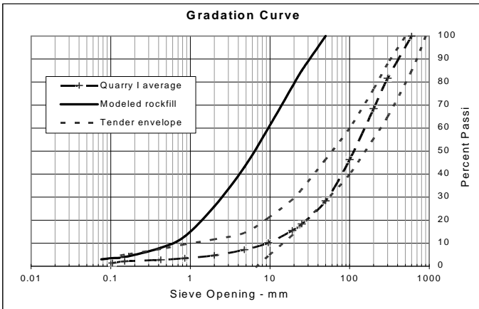
Fig. 2: Modeled rockfill gradation curve
