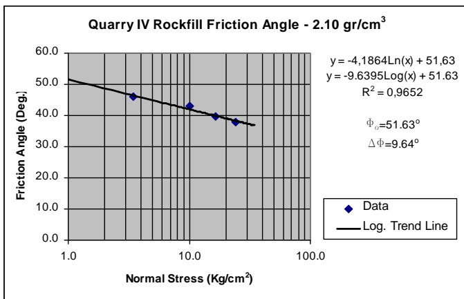
Fig. 4: Variation of the compacted rockfill friction angle v.s normal stress
