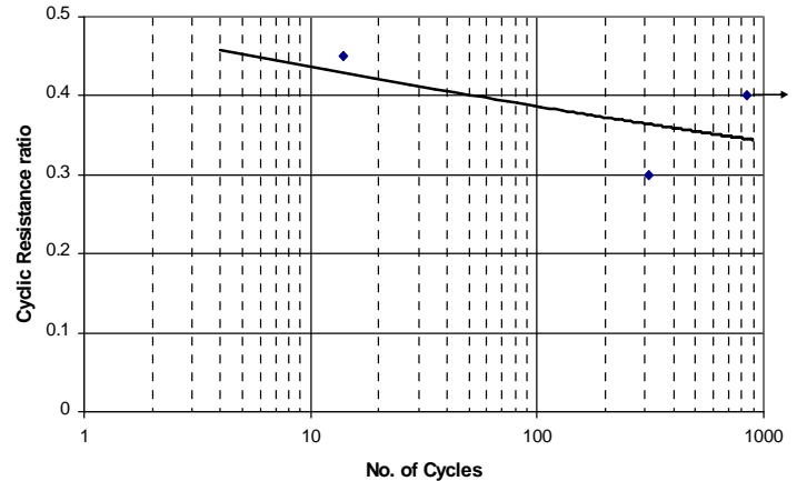
Fig. 6: Cyclic resistance ratio versus number of loading cycles
