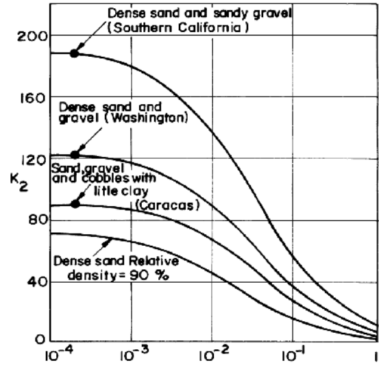
Fig. 8: Values of k_{2max} for gravelly soils (Seed and Idriss, 1970)
