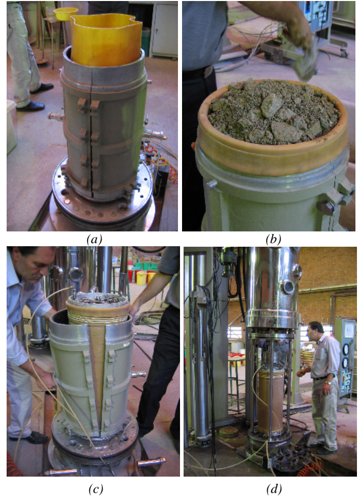
Fig. 3: Specimen preparation: (a) membrane lined split mold, (b) placement of the last material layer, (c) removing the split mold, and (d) placing the specimen inside the triaxial cell
