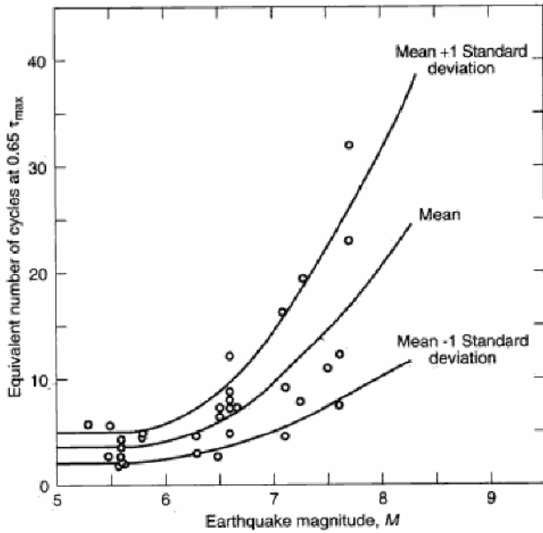
Fig. 5: Equivalent uniform cycles versus earthquake magnitudes (after Seed et al., 1975)
