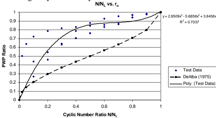
Fig. 7: Cyclic number ratio N/N_L versus pore water pressure ratio r_u
