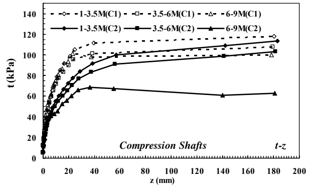
t-z Curve of Compression Shaft
