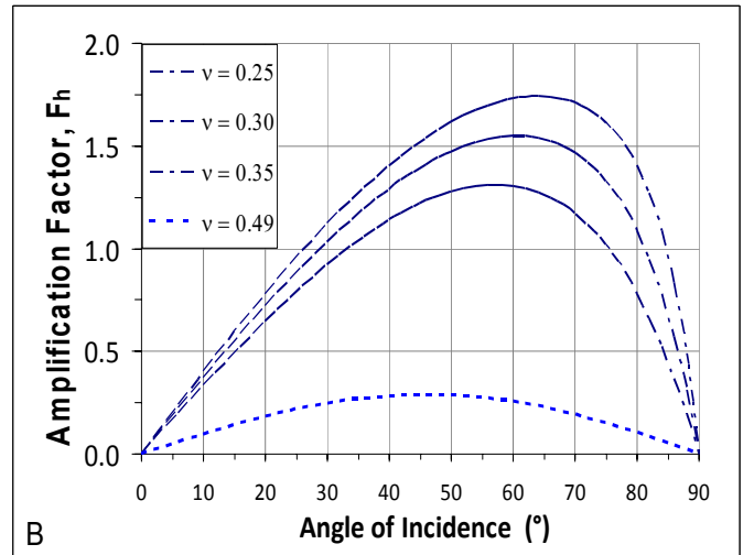
Fig. 13. Variation of vibration amplification factor at free surface of impinging P-wave for different values of Poisson's ratio.
