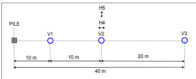
Fig. 17. Arrangement of vibration sensors during driving of the test pile. V1, V2, and V3 indicate "vertical" and H4 and H5 indicate "horizontal" geophones.
