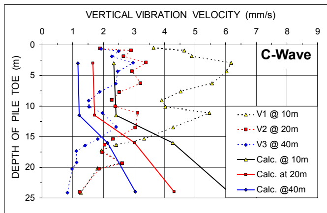
Fig. 28. Measured vertical vibration velocities (dashed lines) and calculated (solid lines) spherical waves (C-waves) emitted
