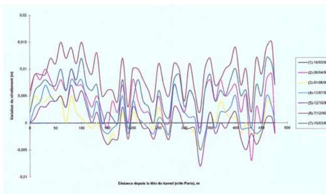
Fig. 5. Leveling defects (track 1, rail 1)
