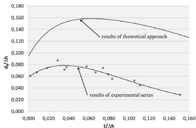
Fig. 12: Results of experimental series as a function of d_f/\Delta h and t/\Delta h in: Schober et. al. (2011), Fig. 12
