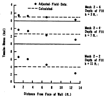
Figure 6. Tensile Stress Distribution Along Reinforcing Mesh (Site 2)
