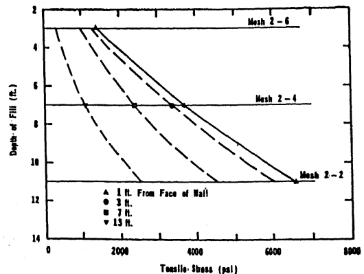
Figure 4. Tensile Stress in Reinforcing Mesh (Site 2)
