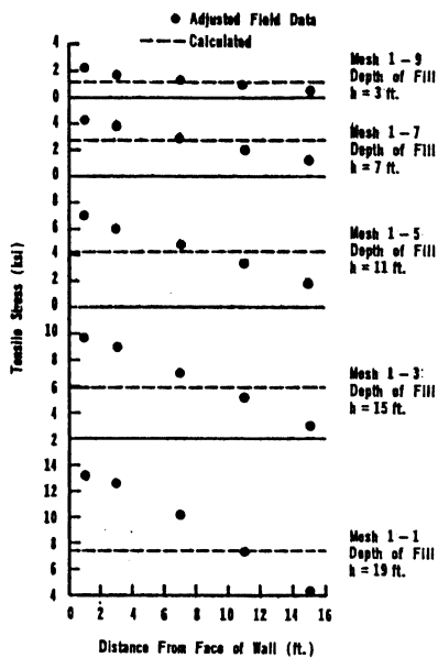
Figure 5. Tensile Stress Distribution Along Reinforcing Mesh (Site 1)
