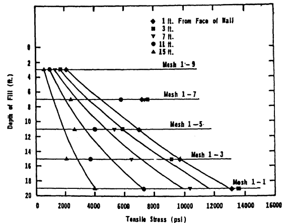
Figure 3. Tensile Stress in Reinforcing Mesh (Site 1)
