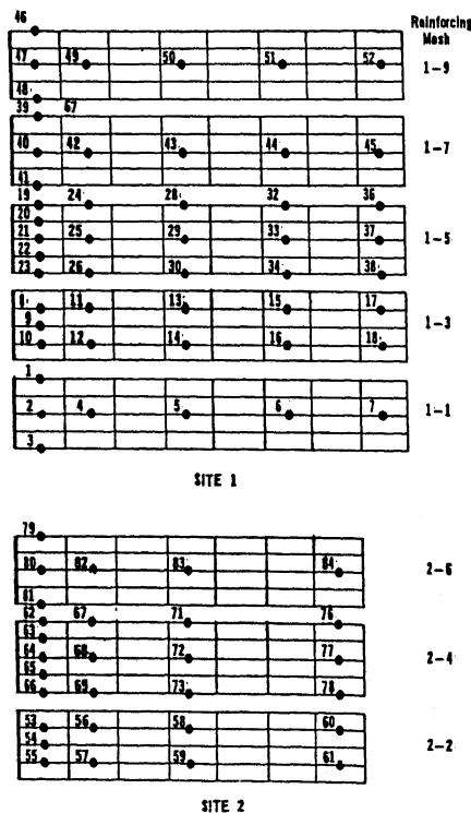
Figure 2. Strain Gage Layout
