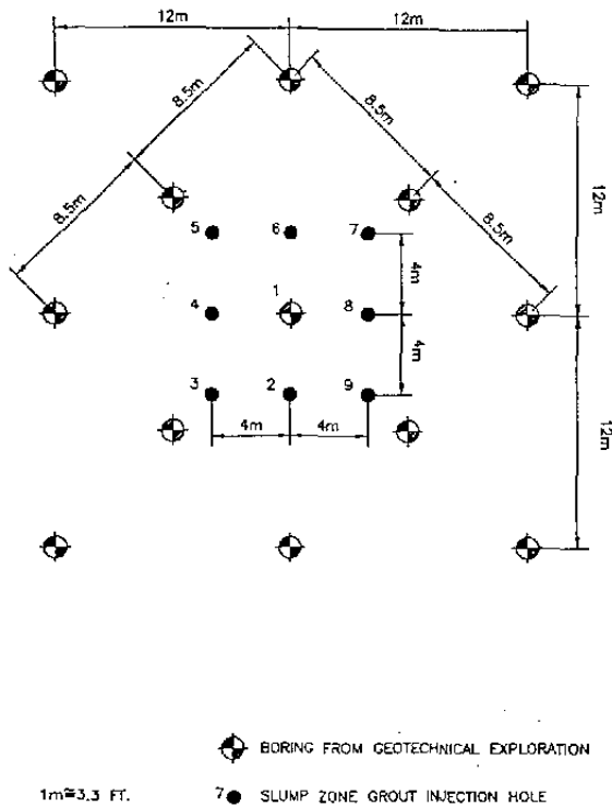
FIGURE 6. PLAN OF TYPICAL EXPLORATION BORING SPACING AND SLUMP ZONE GROUTING PATTERN.
