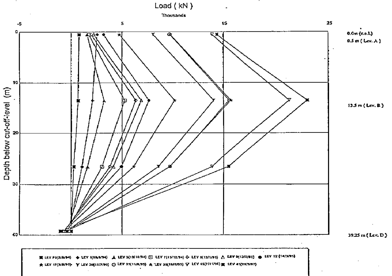
B1-5(SG): LOAD DISTRIBUTION CURVE COMPUTED FROM SGs MEASUREMENT
