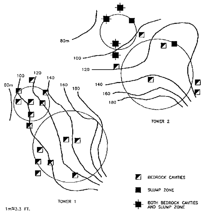
FIGURE 5. PLAN OF BEDROCK DEPTH CONTOURS AND GROUND IMPROVEMENT LOCATIONS NTS
