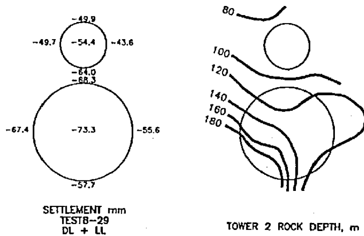
FIG. 16. Tower 2 Settlement Map and Rock Contour Plan
