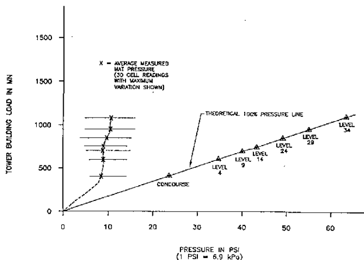
RELATION OF AVERAGE MAT PRESSURE CELL READINGS AND BUILDING LOAD
