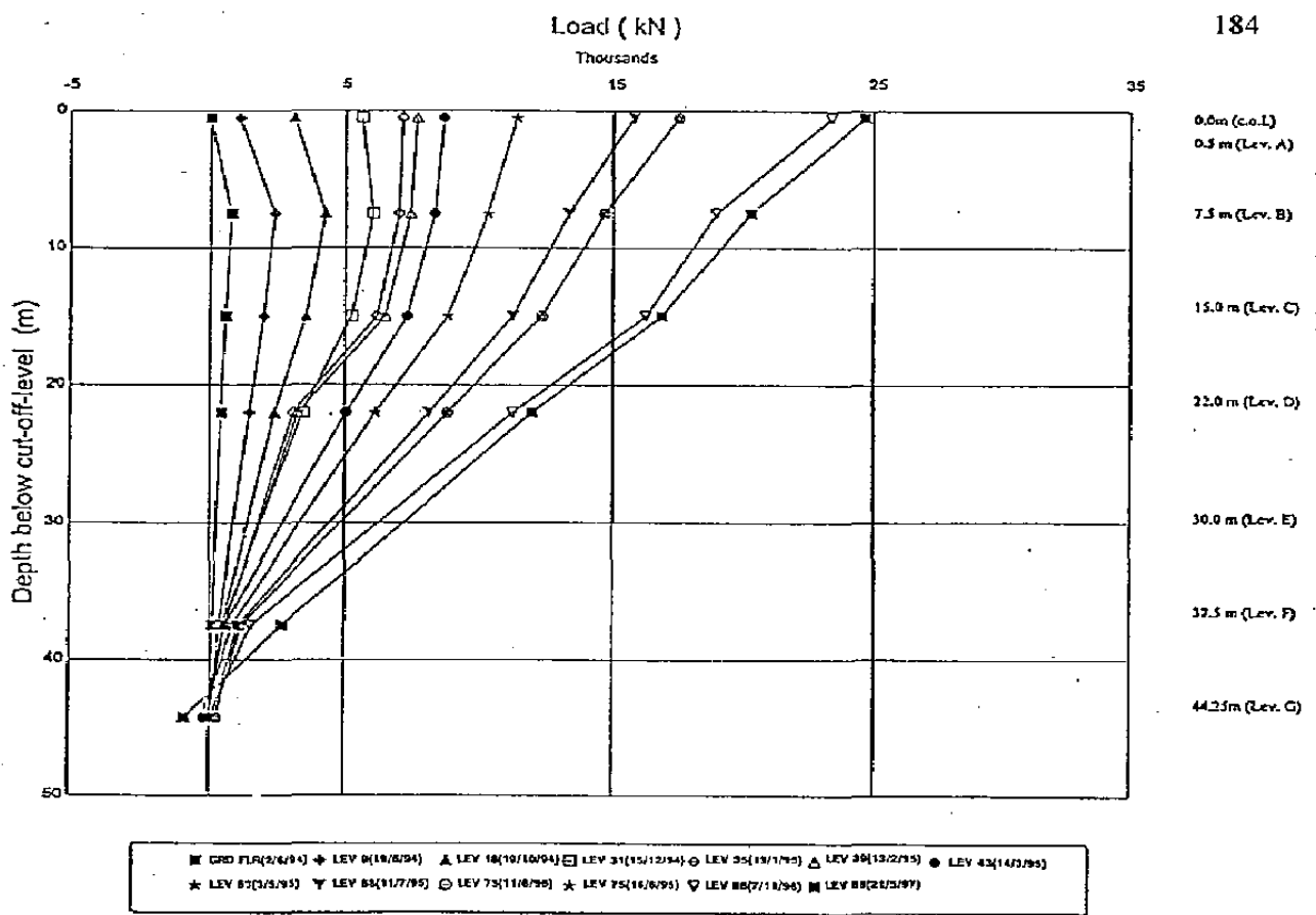
T1-1A(SG): LOAD DISTRIBUTION CURVE COMPUTED FROM SGs MEASUREMENT
