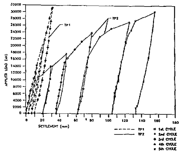
FIG. 3 RELATIONSHIP BETWEEN APPLIED LOAD WITH SETTLEMENT (TRANSDUCER) - TP1 AND TP2
