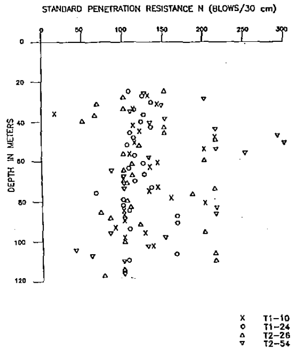
FIG. 3. Standard Penetration Resistance Profile
