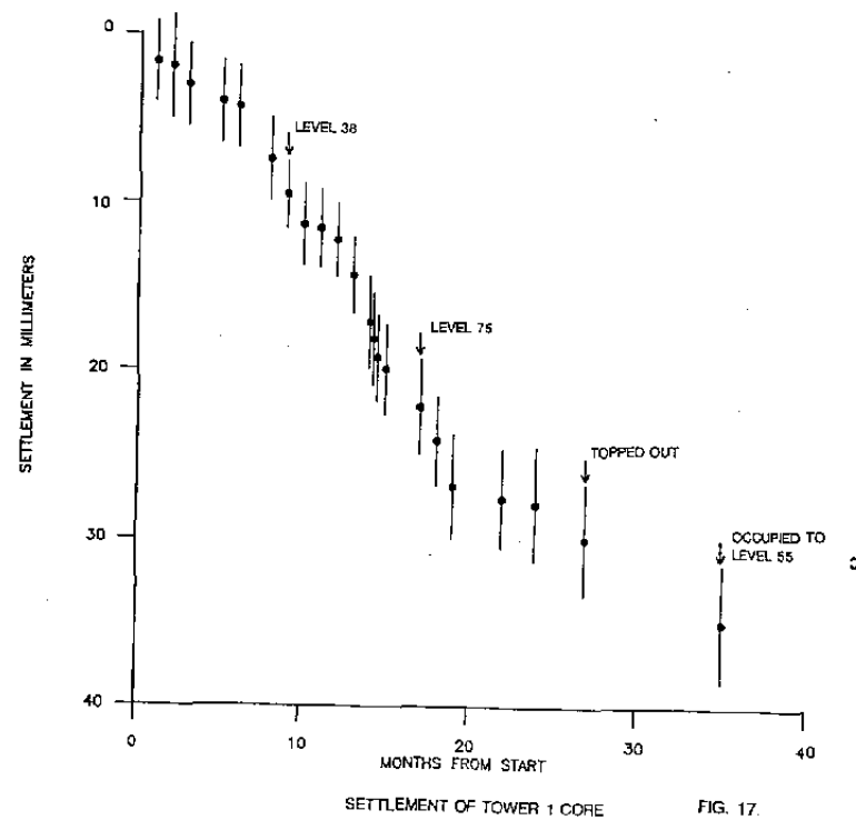
SETTLEMENT OF TOWER 1 CORE FIG. 17
