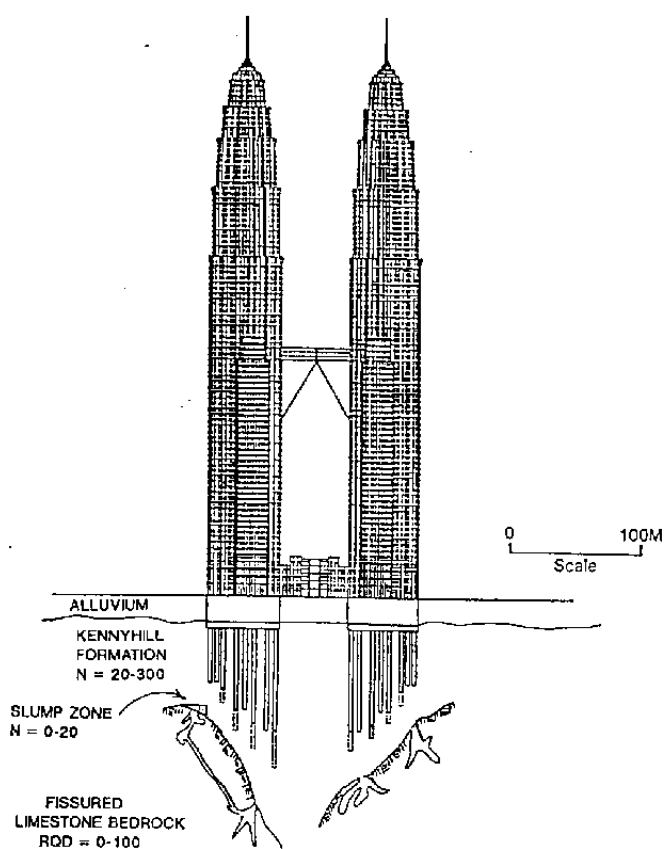
FIG. 1 TOWER FOUNDATION PROFILE
