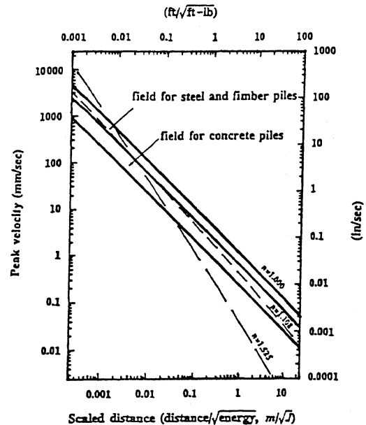
Fig.1 Peak ground velocity versus scaled distance for pile driving
