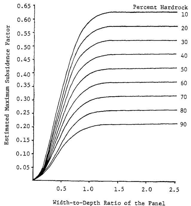
Figure 5. Determination of the Maximum Subsidence Factor from the Width-to-Depth Ratio and the Percent of Hardrock
