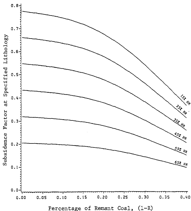
Figure 6. Effect of Extraction Ratio and Lithology on S_{max} : Supercritical Data Analysis
