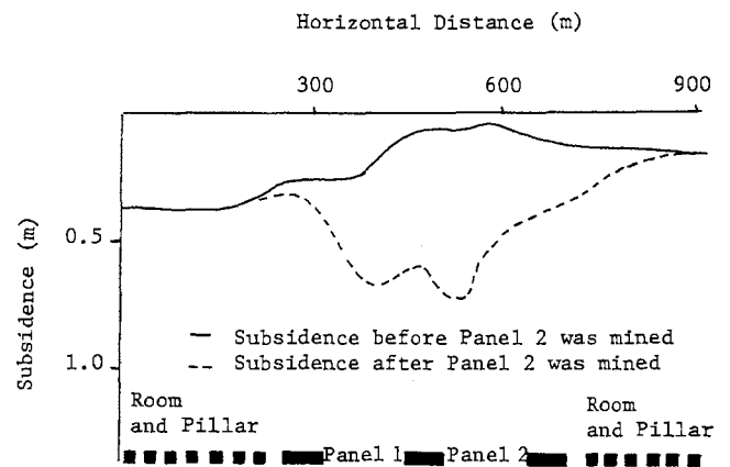
Figure 2. Transverse Profiles of a Case Study Showing the Influence of the Adjoining Room and Pillar Sections
