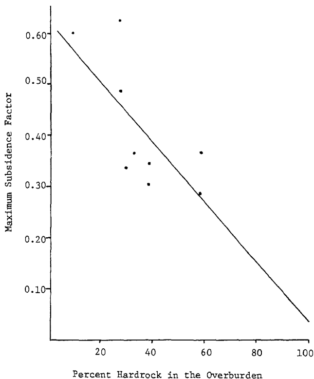
Figure 4. The Influence of Sandstone and Limestone in the Overburden on the Subsidence Factor for Critical and Supercritical Extractions
