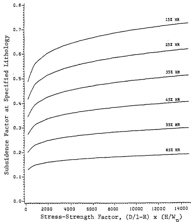
Figure 7. Effect of Pillar Stress-Strength and Lithology on S_{max} : Supercritical Data Analysis
