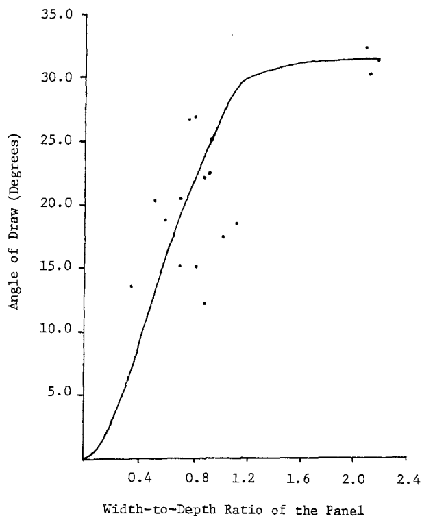
Figure 3. The Influence of the Width-to-Depth Ratio on the Angle of Draw
