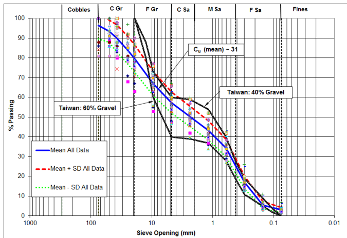
Fig. 5. Study Site and Taiwan Gravel Grain Size Distributions
