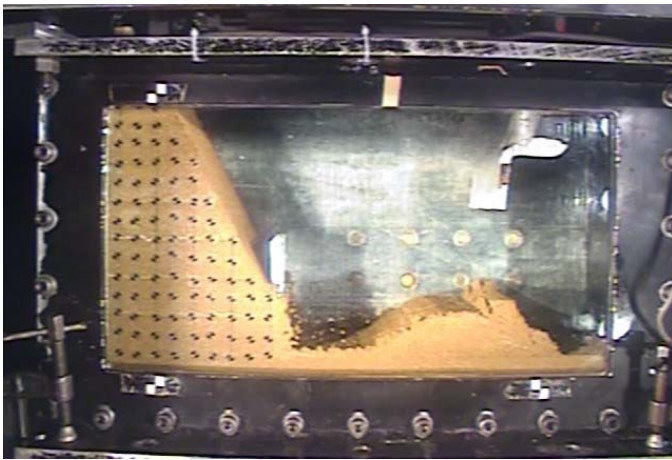
(b) After 1.4 m excavation
