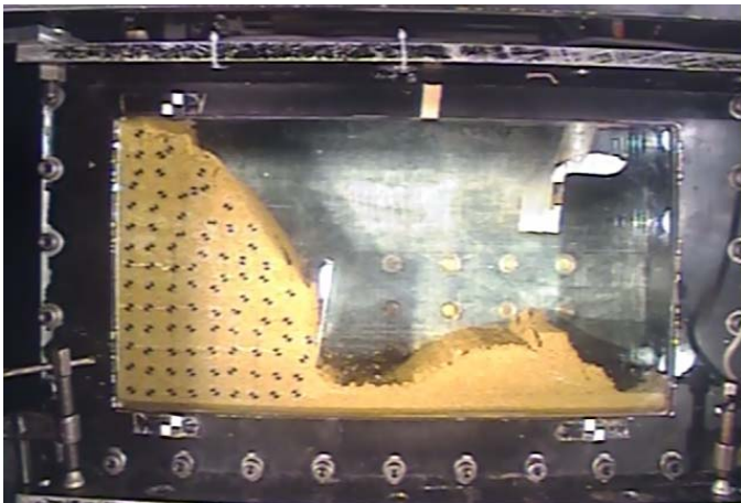
(c) Failure at 36 g
