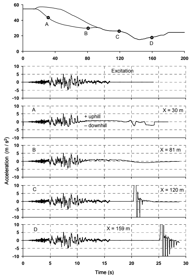
Fig. 19. Acceleration time histories at selected point along the sliding surface of the Nikawa landslide.
