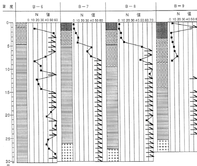
Fig. 4. Geotechnical cross section, along with NSPT blows on boreholes that were conducted after the slide [courtesy of Professor K. Sassa]
