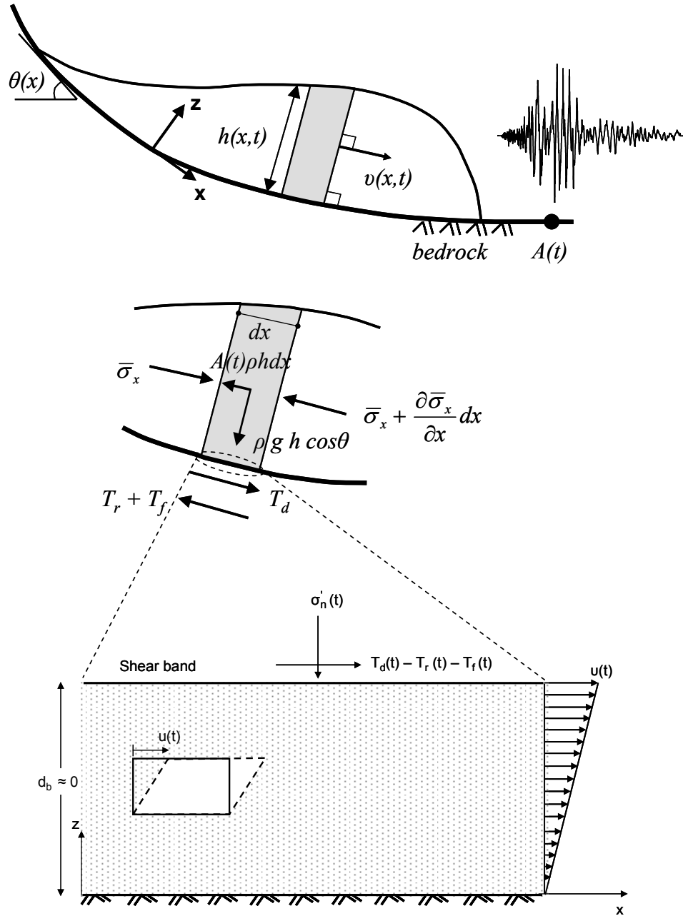
Fig. 10. 1 dimensional depth-integrated model for the analysis of earthquake-induced landslide evolution. Stress equilibrium is referred to a local coordinate system that is fitted to the underlying topography.
