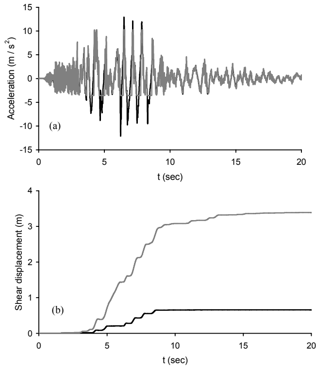
Fig. 12. (a) Input (Record NIG019 2004: PGA = 1.3 g ) and response acceleration time histories at the base of the landslide (black line), and at the soil wedge (gray line) for case b (sliding surface within an assumed thin silt layer), and (b) computed time histories of relative shear displacements, for sliding surface: (i) within the sand layer (no grain crushing is considered, max_u = 0.65 m ) (black line), and (ii) within an assumed thin silt layer at the top of the siltstone ( max_u = 3.4 m ) (gray line)
