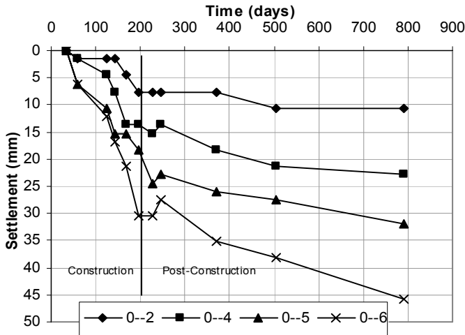
Fig. 6. Settlement of the gefoam approach fill, East Array.
