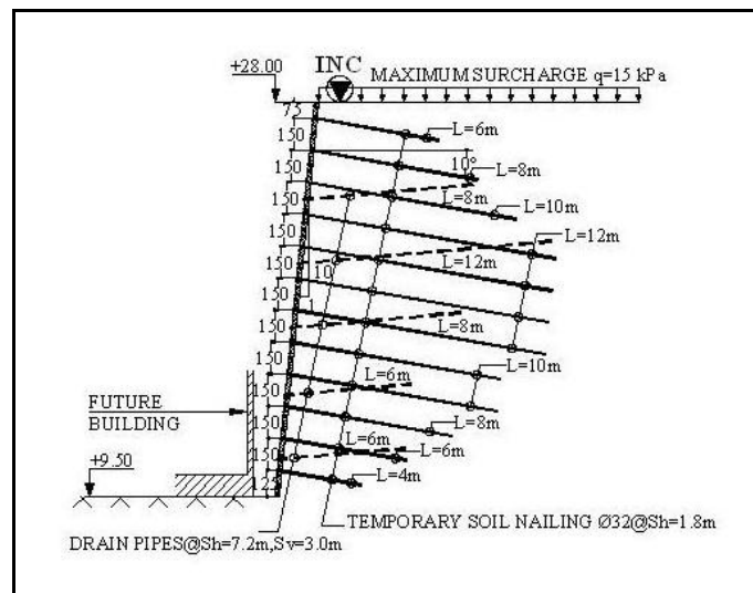
Fig. 11a. Detailed cross-section of Type 4
