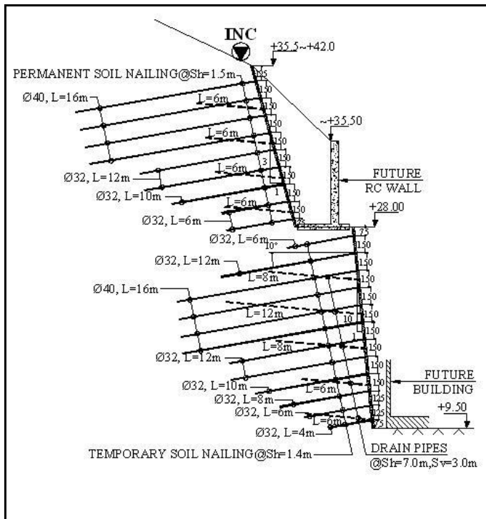
Fig. 10b. Detailed cross-section of Type 3
