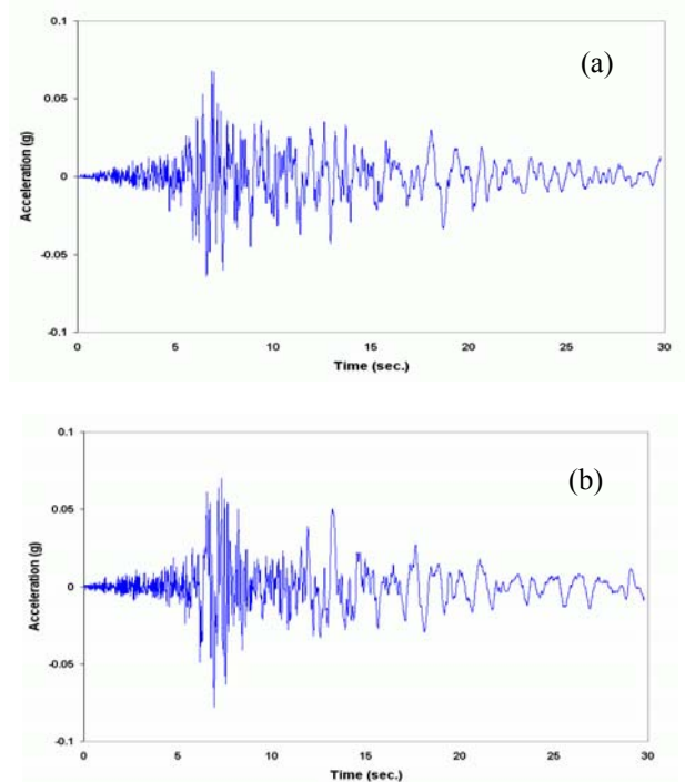
Fig. 6 Recorded Acceleration Time Series at a Depth of 7.5 m at the Wildlife Site (During the 1987 Elmore Ranch Earthquake) (a) EW; (b) NS
