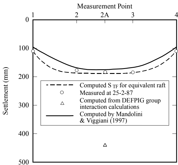
Fig. 24. Computed and measured settlements along edge of silo.
