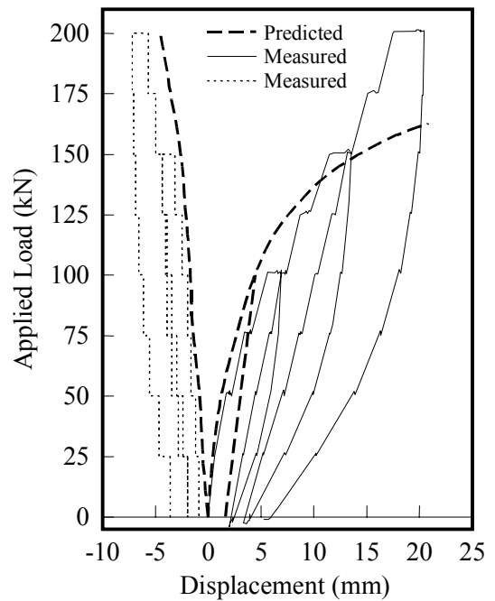
Fig. 10. Measured and predicted lateral load versus deflection – pile P2(H).
