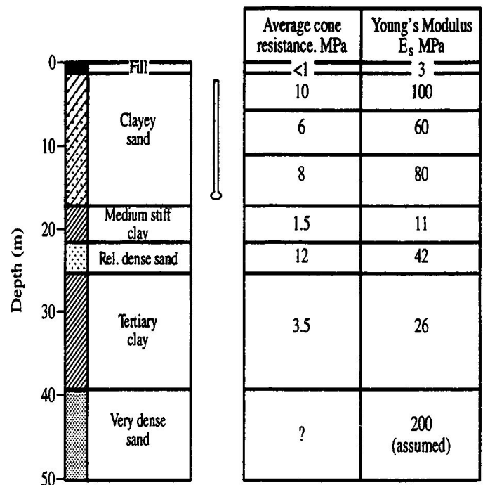
Fig. 23. Geotechnical profile and model for case of Goosens and van Impe (1991).
