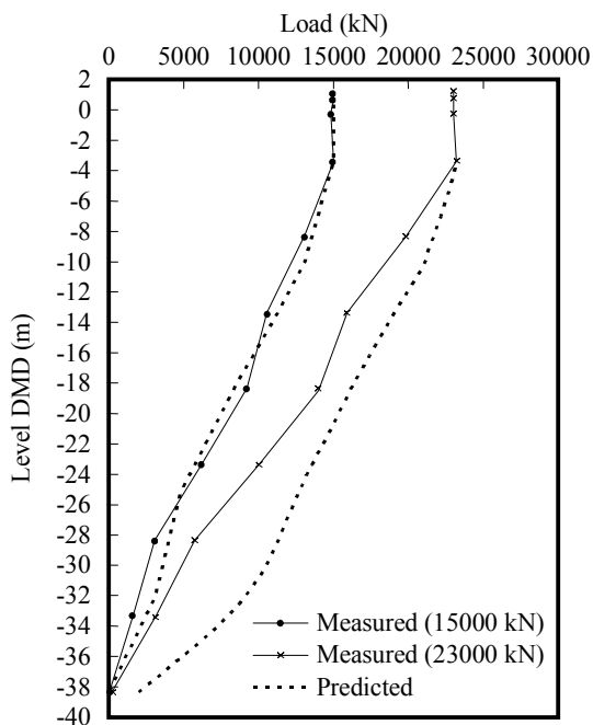
Fig. 6. Predicted and measured axial load distribution for pile P3(H).
