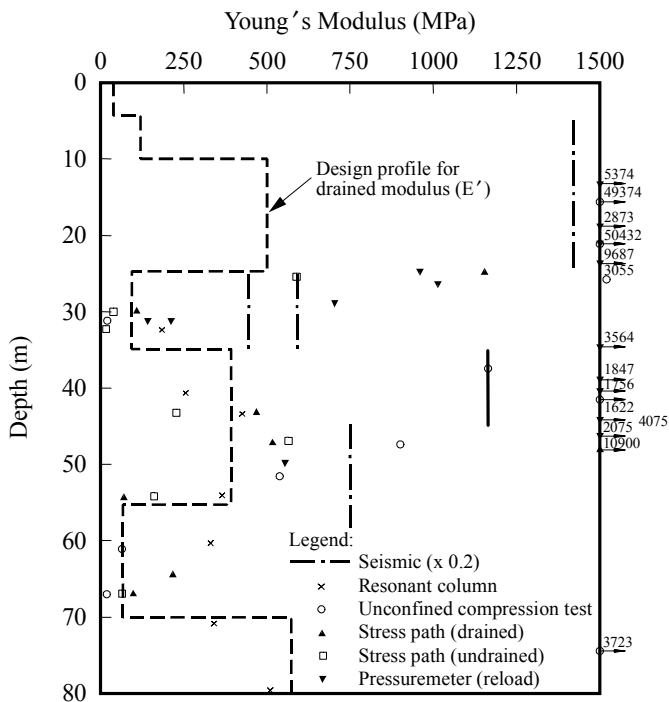
Fig. 1. Emirates project – summary of Young's Modulus values.
