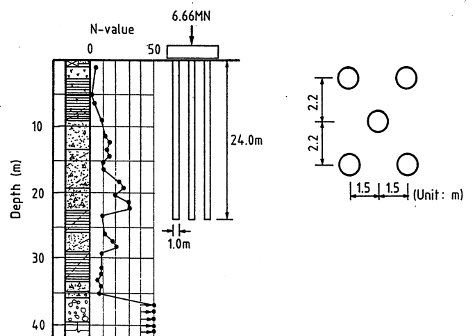
Fig. 15. Soil profile for case history of Kaino & Aoki (1985).
