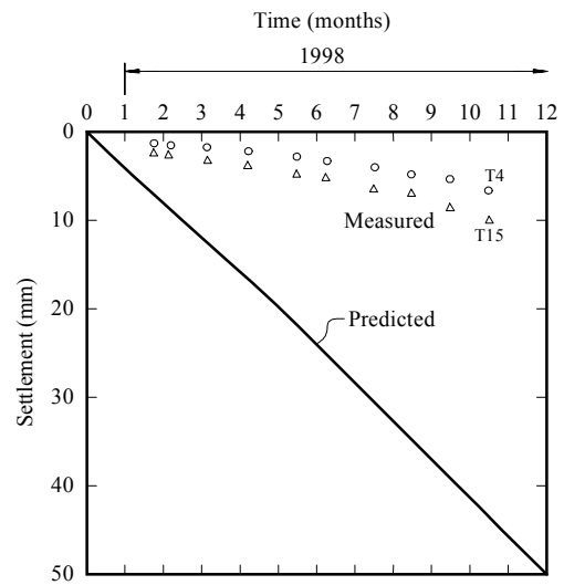
Fig. 20. Predicted and measured settlement vs time – Hotel Tower.
