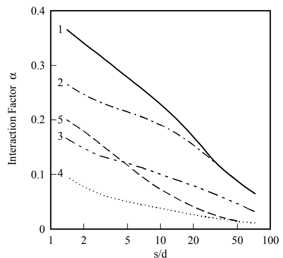
Fig. 22. Sensitivity of computed interaction factors to analysis assumptions.
