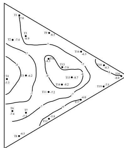
Fig. 21. Measured settlement contours – Hotel Tower.
