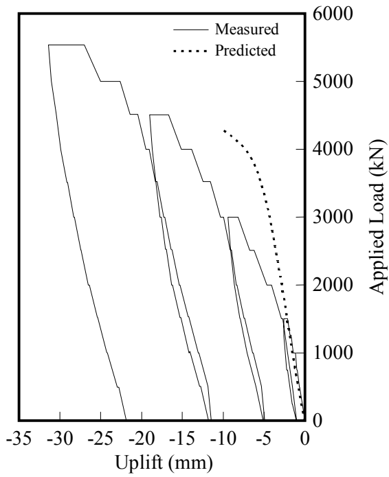
Fig. 7. Predicted and measured load-uplift behaviour for tension test on pile P1(H).
