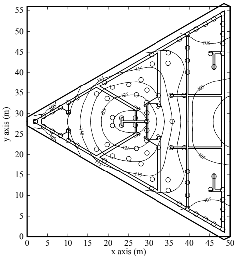
Fig. 18. Foundation layout and computed settlement contours for Hotel Tower.
