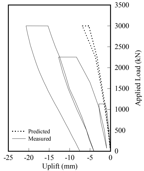
Fig. 9. Measured and predicted load-uplift behaviour for cyclic uplift test- pile P2(H).
