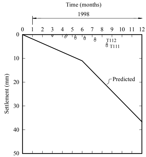
Fig. 19. Predicted and measured settlement vs time – Office Tower.
