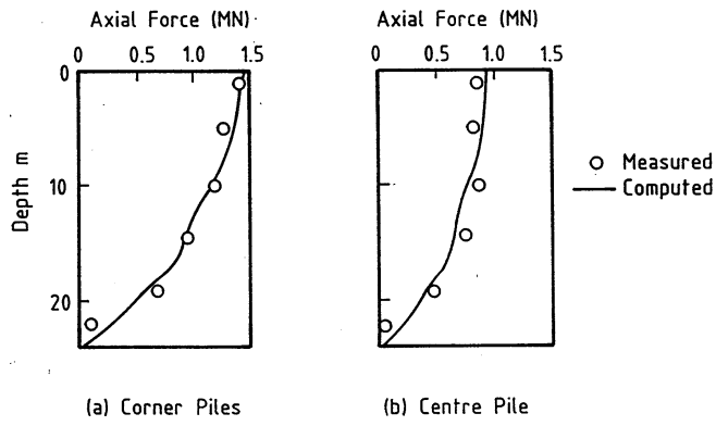
Fig. 16. Measured and computed load distributions along piles.
