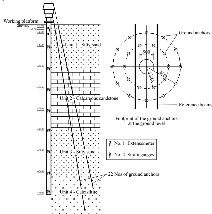
Fig. 4. Setup for compression pile tests.
