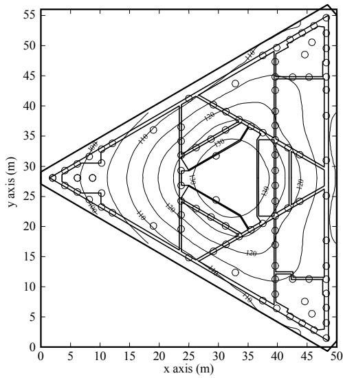
Fig. 17. Foundation layout and computed settlement contours for Office Tower.
