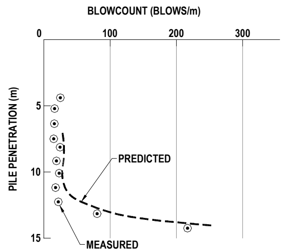
Fig. 14. Predicted blowcount during driving.
