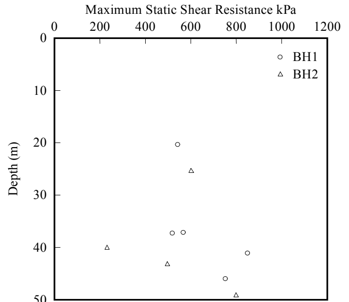
Fig. 2. Summary of ultimate shaft friction from CNS tests.
