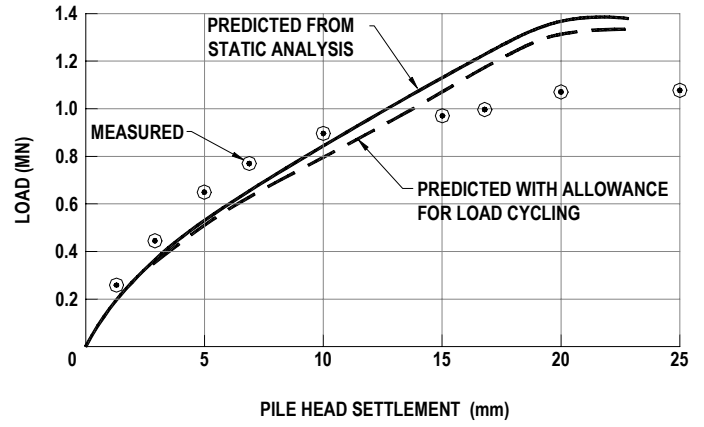
Fig. 13. Predicted load-settlement behaviour for pile head.
