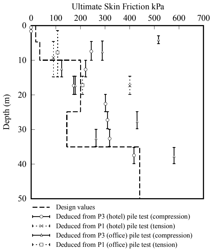
Fig. 8. Ultimate skin friction values – design values and values derived from load tests.
