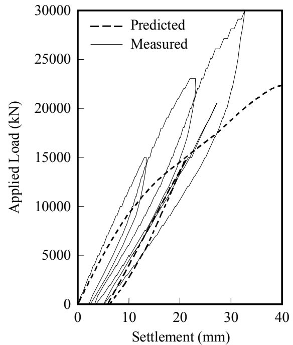
Fig. 5. Predicted and measured load-settlement behaviour for pile P3(H).
