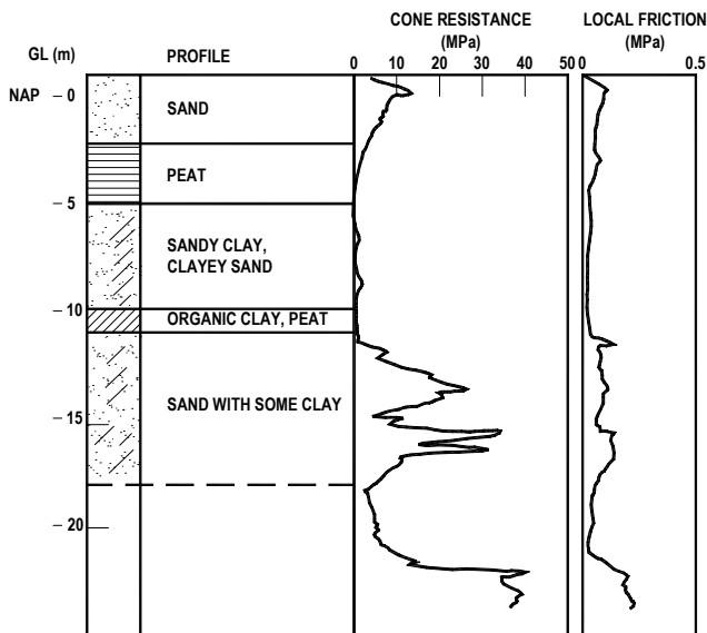
Fig. 12. Soil profile and cone penetration data for ESOPT II case.
