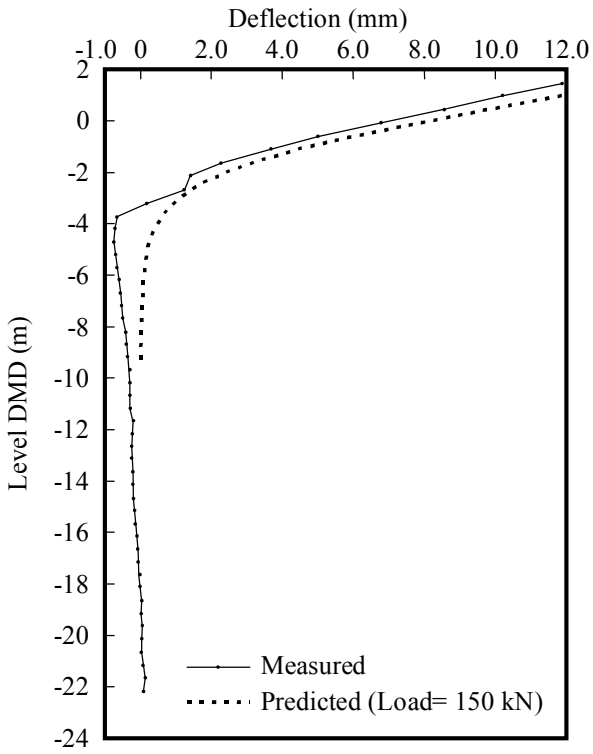
Fig. 11. Measured and predicted deflection distributions – pile P2(H).
