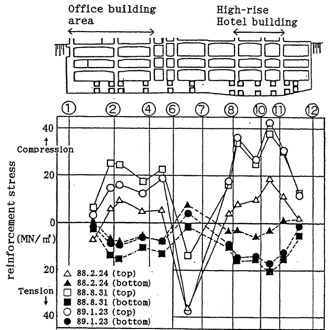
Fig-9 Measured distribution of reinforcing bar stress
