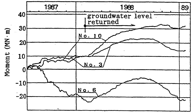
Fig-8 Development of bending moment in foundation beam
