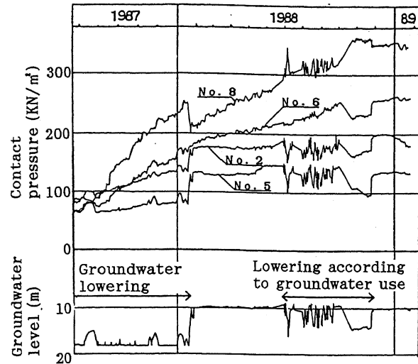
Fig-5 Measured contact pressure and groundwater level
