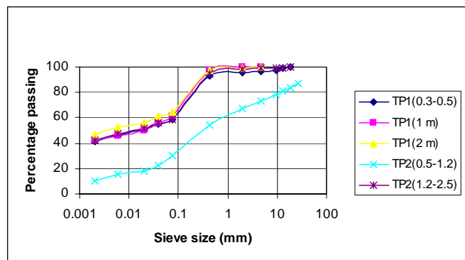
Fig. 11: Particle size distribution of test pit samples
