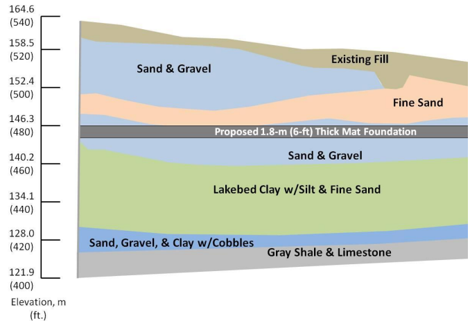
Fig. 3. Generalized Subsurface Profile
