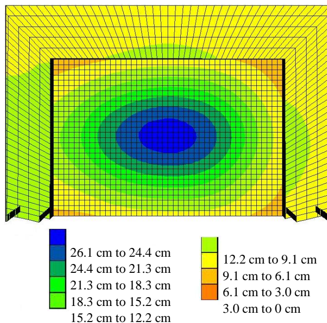
Fig. 6. Settlement Contours – Mat Foundation Only
