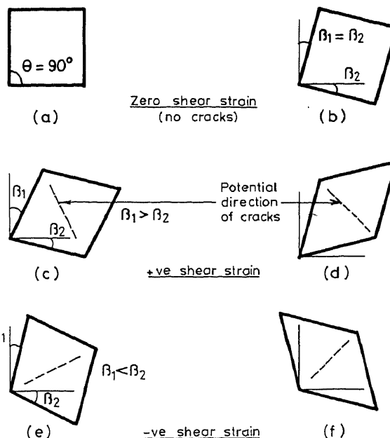
Fig.5 Wall Distortion and Potential Direction of Cracks
