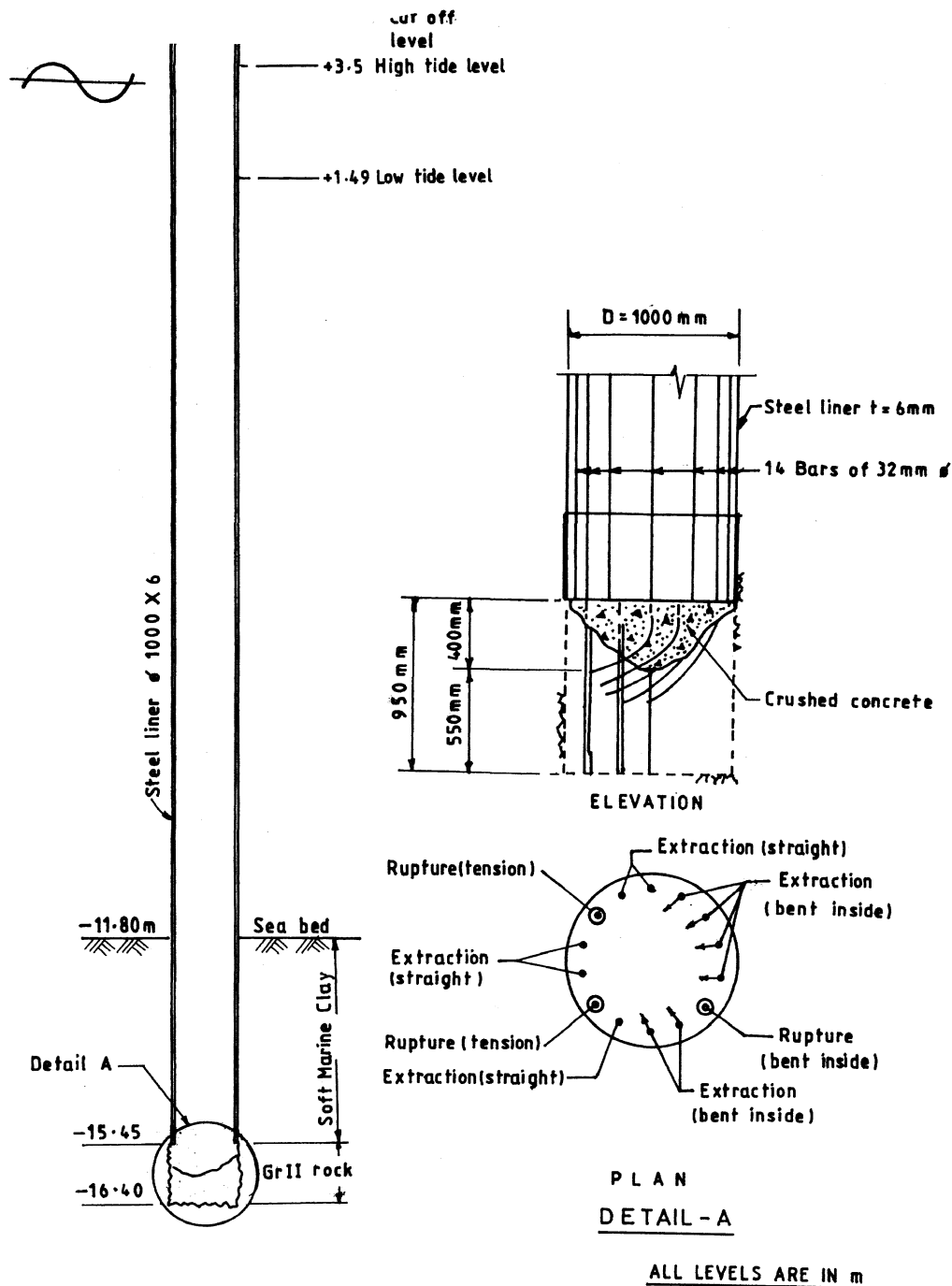
FIG.1. DETAILS OF DAMAGED PILE
