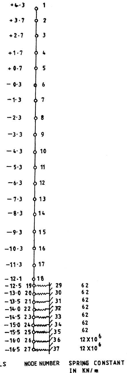
FIG.3. DISCRETISATION OF 760 mm PILE.
