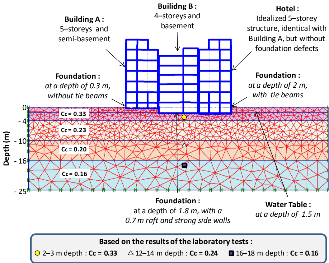
Fig. 6. Finite element modeling of the three neighboring buildings.
