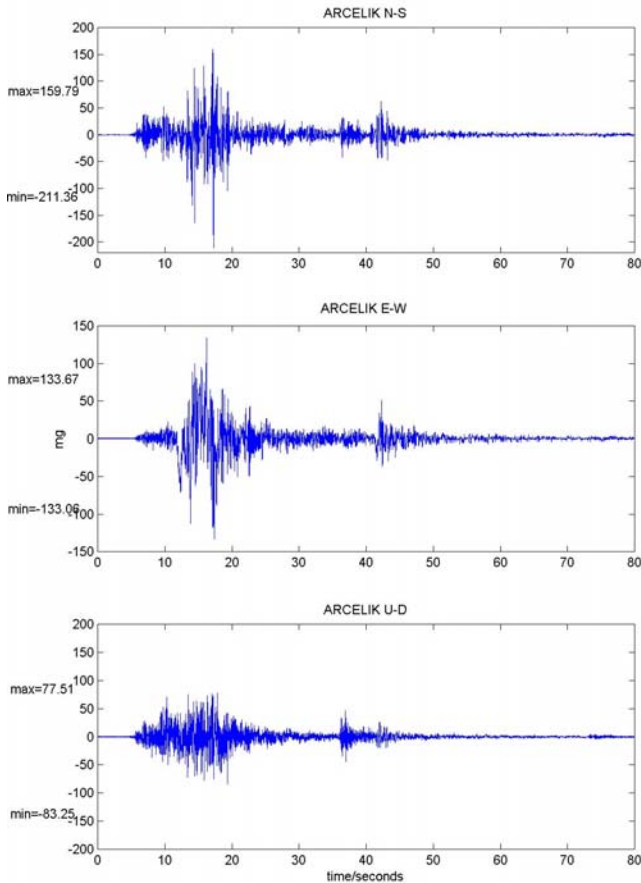
Fig.1 The acceleration time history of ARC station (Kocaeli Earthquake).
