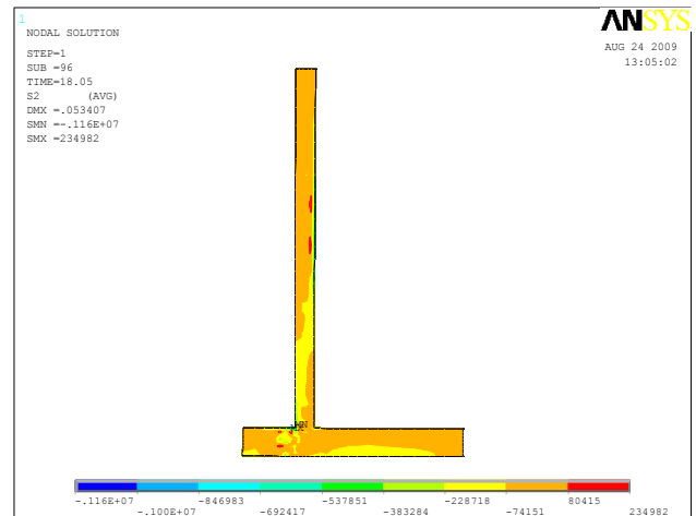
Fig. 12. Stress distibution during Kobe Earthquake.
