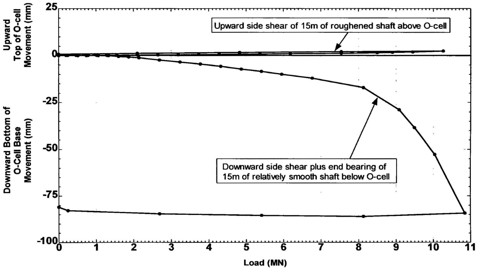
Fig. 5 - Example 561, effect of wall roughening
