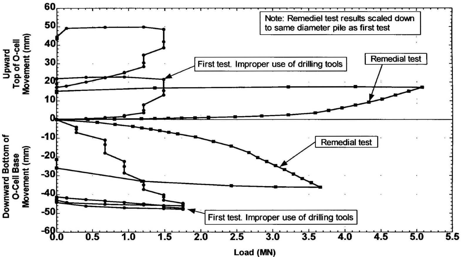
Fig. 6 - Example 562, improper use of drilling tools
