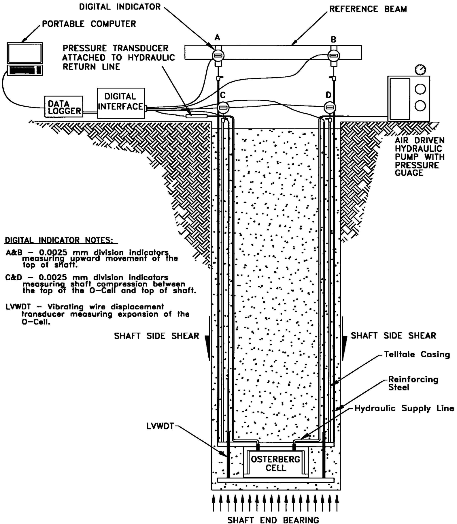
Fig. 2 Typical Osterberg cell test instrumentation
