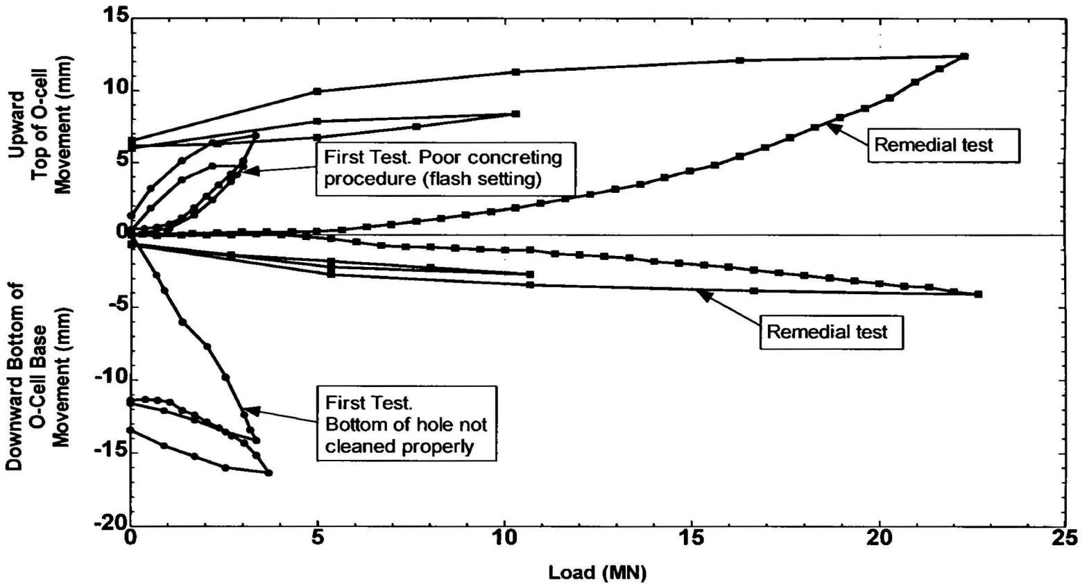
Fig. 8 - Example 723, effect of poor cleanout procedures in weathered rock (EB) and effect of poor concreting procedures (SS)
