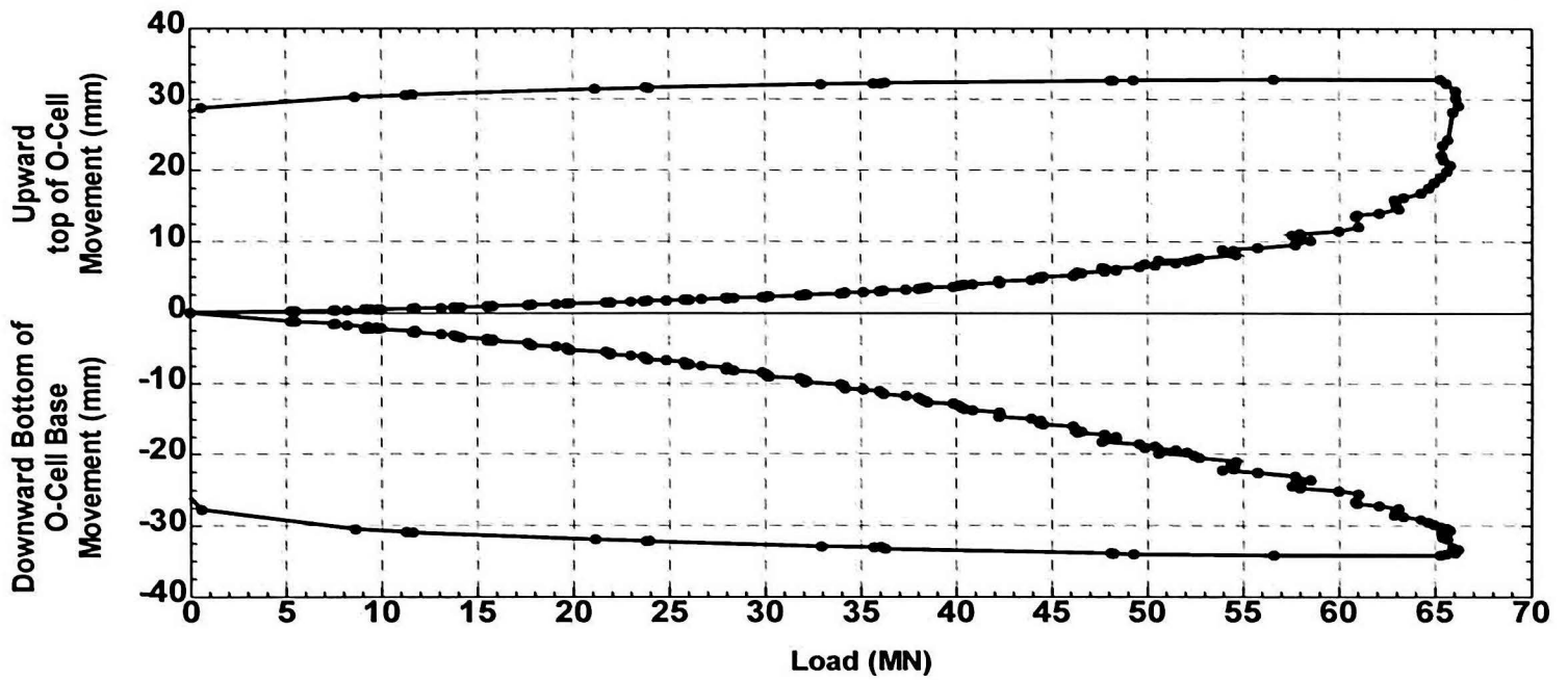
Fig. 9a - Osterberg cell load-movement curves, world record load test (2.75m diameter shaft embedded in limestone)
