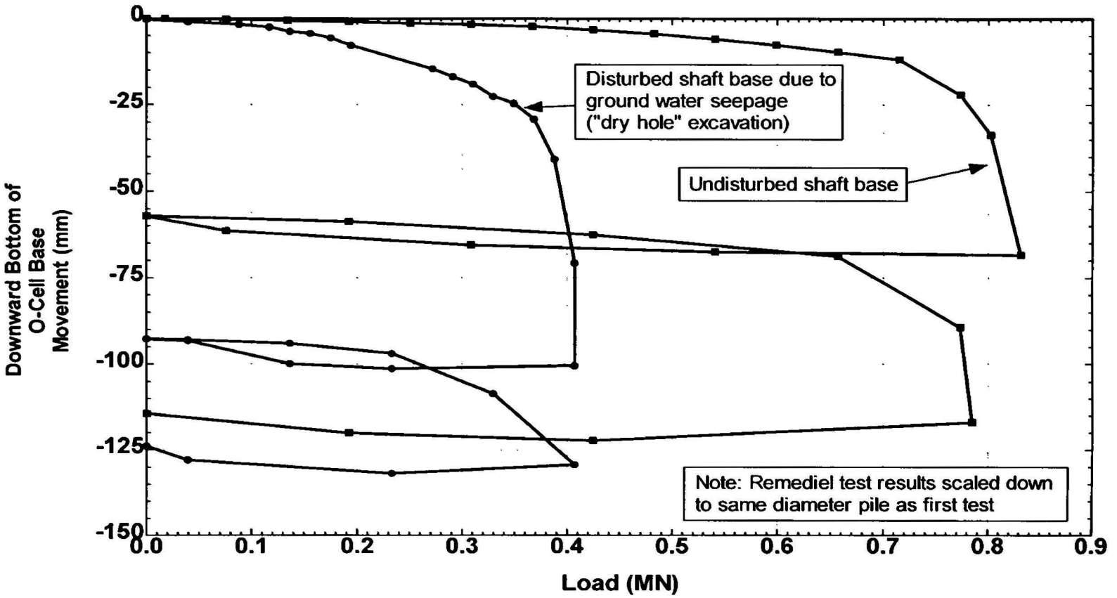
Fig. 7 - Example 643, effect of poor cleanout procedures ("dry hole") in clay
