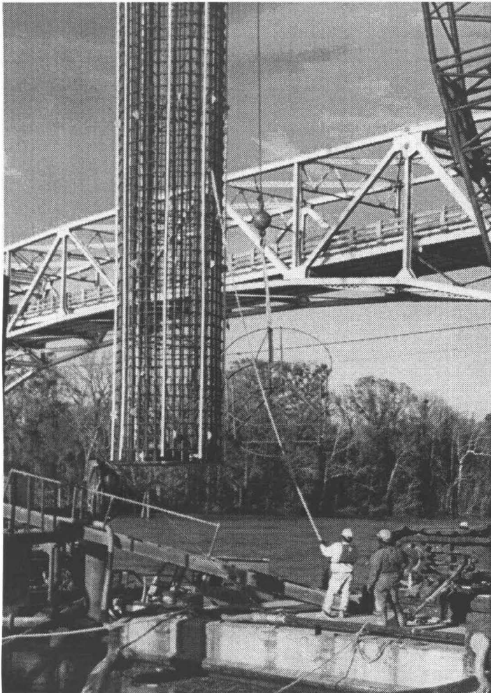
Fig. 9b - world record test shaft installation with three O-cells attach (162 MN combined capacity).
