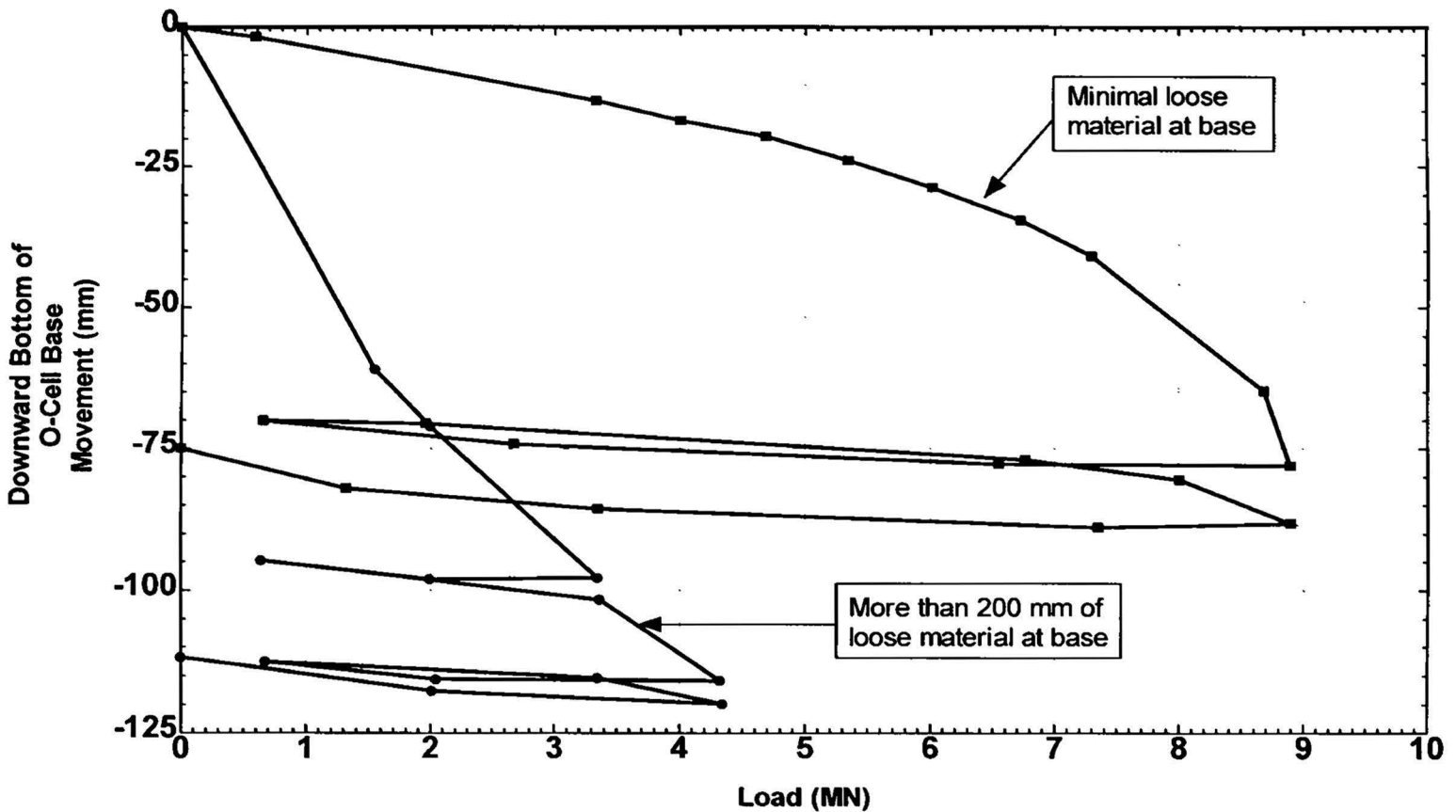
Fig. 4 - Example 502, effect of poor cleanout ("dry hole") in sands, gravel
