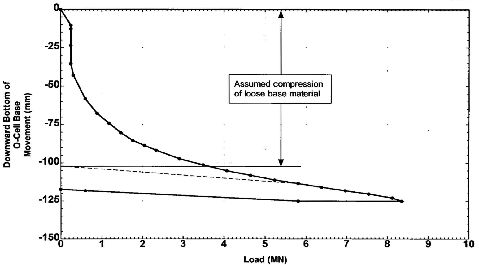
Fig. 3 - Example 272, effect of poor cleanout procedures ("dry hole") in weathered rock
