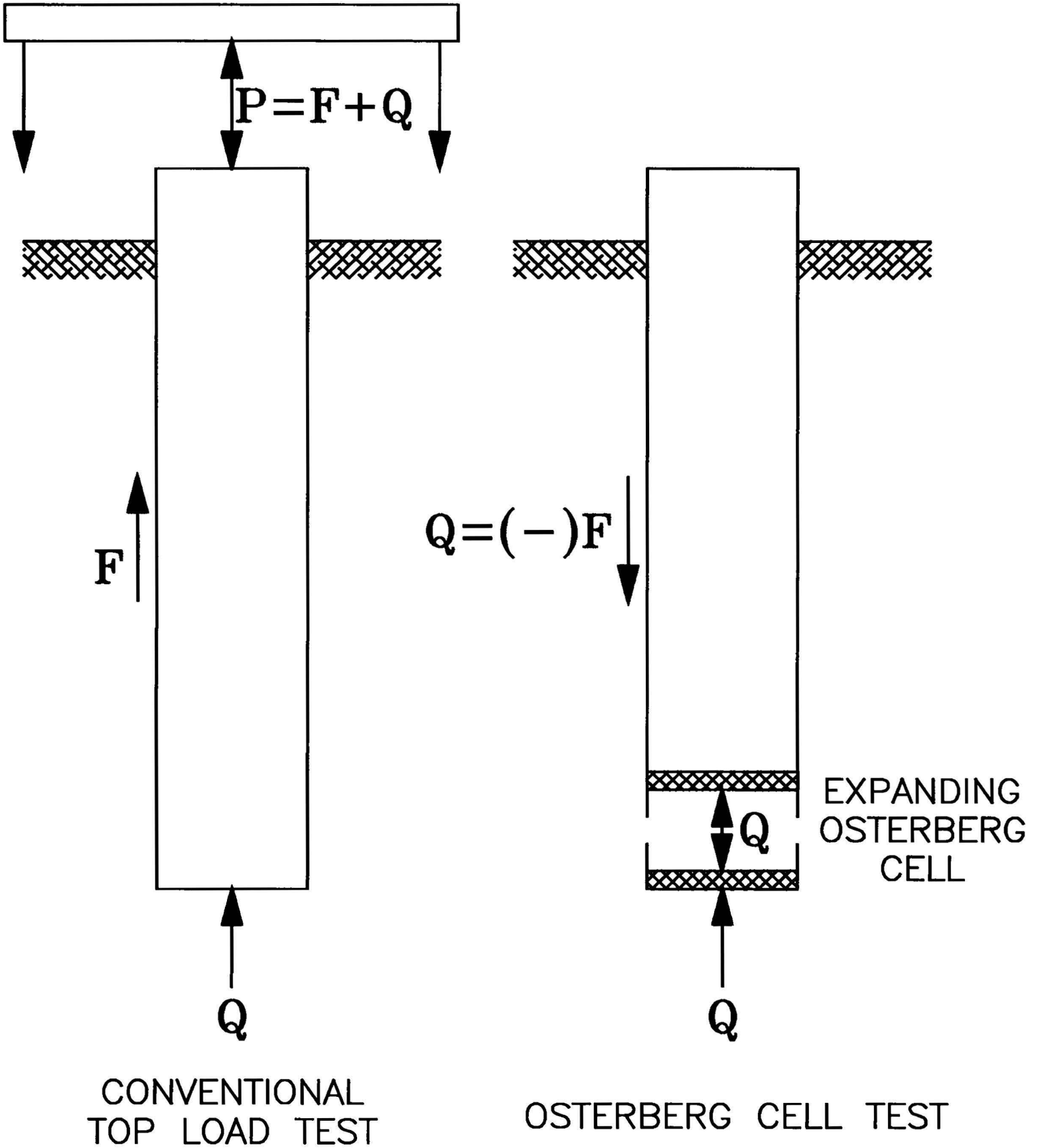
Fig. 1 Schematic comparison of conventional top load test and Osterberg cell test
