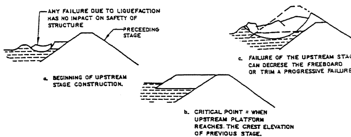
Figure 4. Possible Consequences of Upstream Stage Failure
