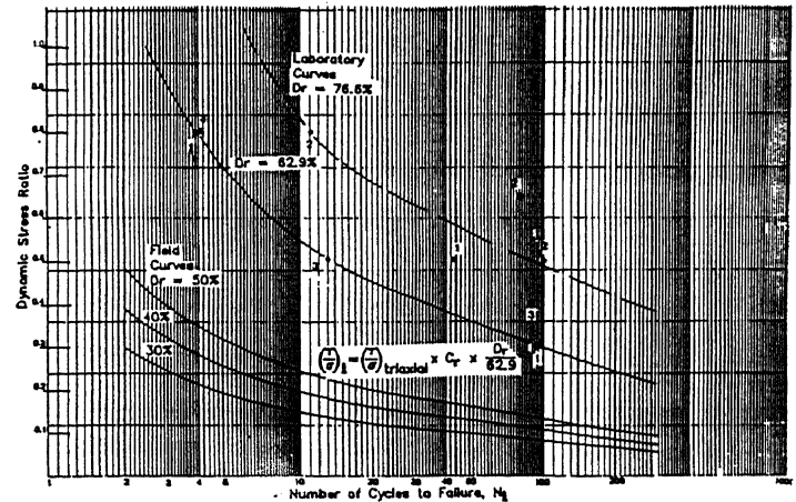
Figure 5. Results of Dynamic Triaxial Tests
