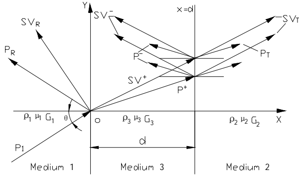
Fig.1. The propagation model of plane P wave in three mediums
