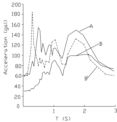
Fig.7. Acceleration response spectra for area A and area B in Tianjin, China [after Zhou, Wang and Han, 1984]
