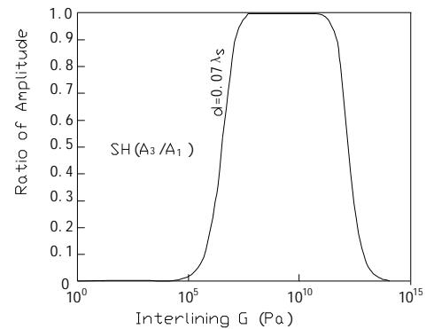
Fig.5. Pertinent curves of the amplitude rate of transmission wave and interlining medium shear modulus G (incident angle \theta=45^\circ )
