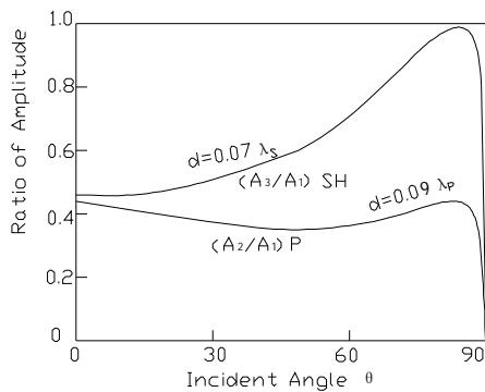
Fig.3. Pertinent curve of amplitude rate of transmission wave and incident wave with incident angle
