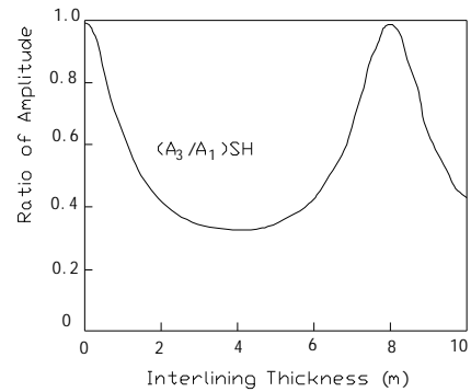
Fig.4. Pertinent curves of the amplitude rate of transmission wave and interlining medium thickness (incident angle \theta=45^\circ )
