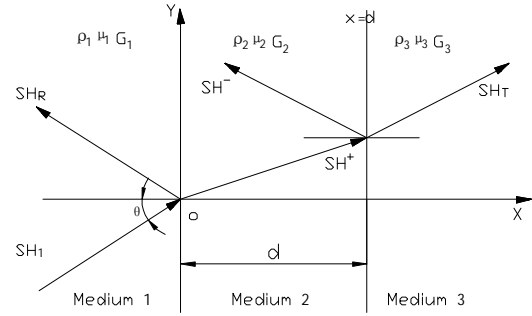
Fig.2. The propagation model of plane SH wave in three mediums
