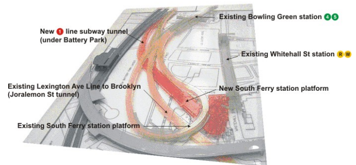
Fig. 2. Project Location – New Tunnel Configuration [Source: MTA 2006]
