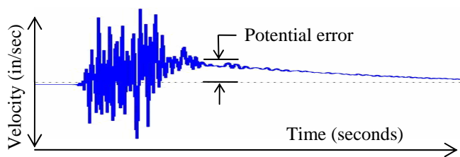
Fig. 5. Waveform, example of faulty seismograph reading
