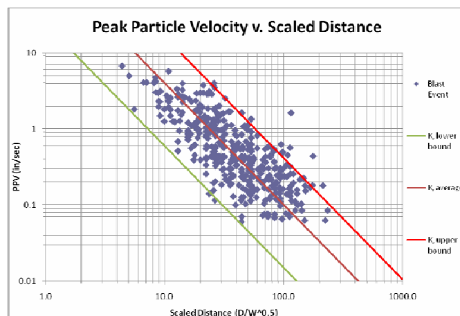
Fig. 11. Scaled distance log-log plot of data
