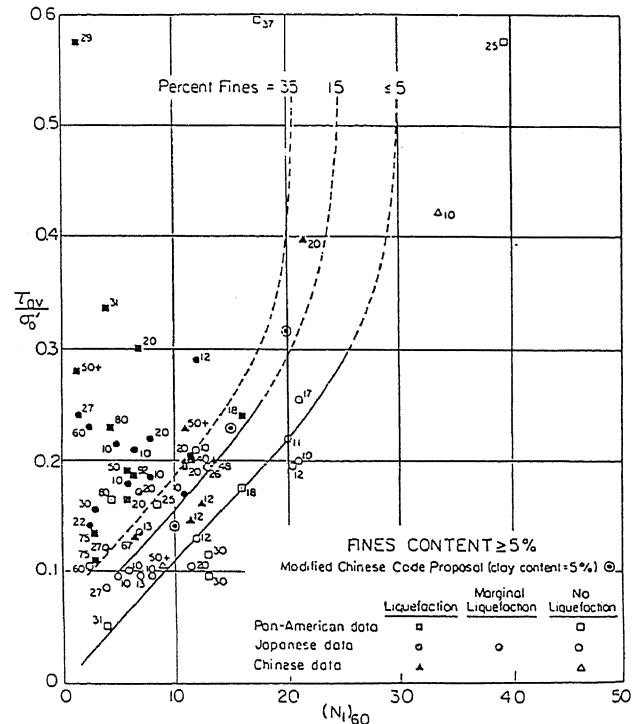
Figure 3. Relationships between stress ratios causing liquefaction and N_1 -values for silty sands for M=7-1/2 earthquakes (after Seed, Tokimatsu, Harder, and Chung, 1985)
