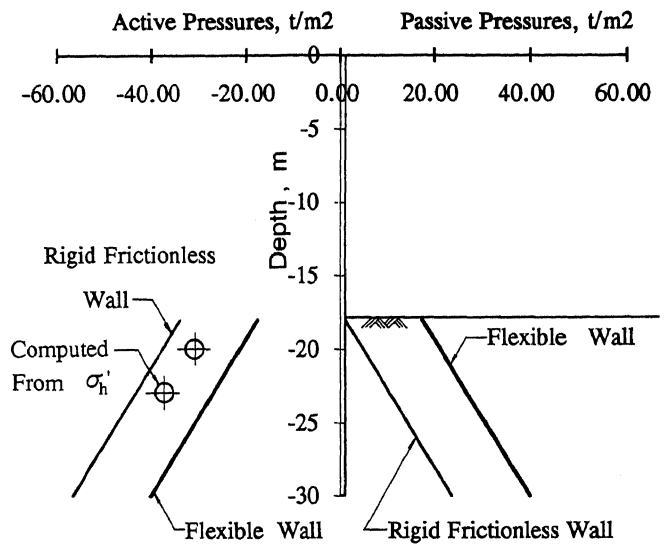
Figure 9 Computed Vertical Pressures
