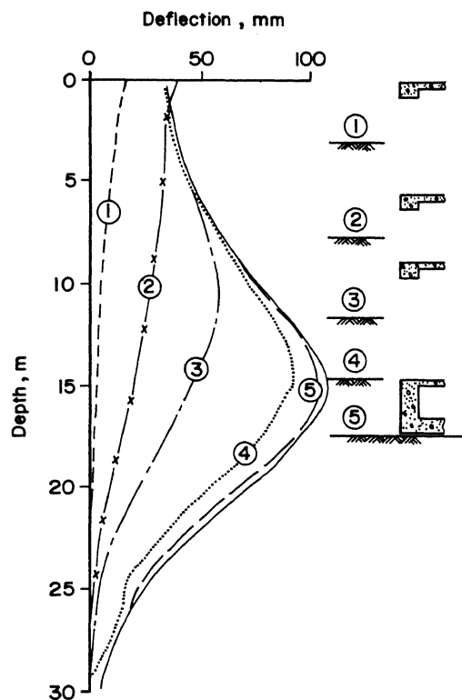
Figure 5 Wall Deflections During Excavation
