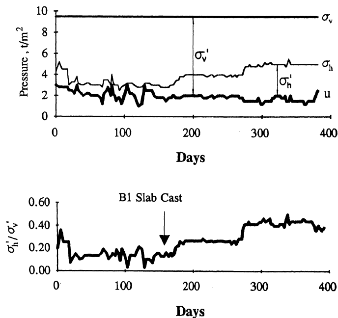
Figure 7 Active Pressures at a Depth of 5m
