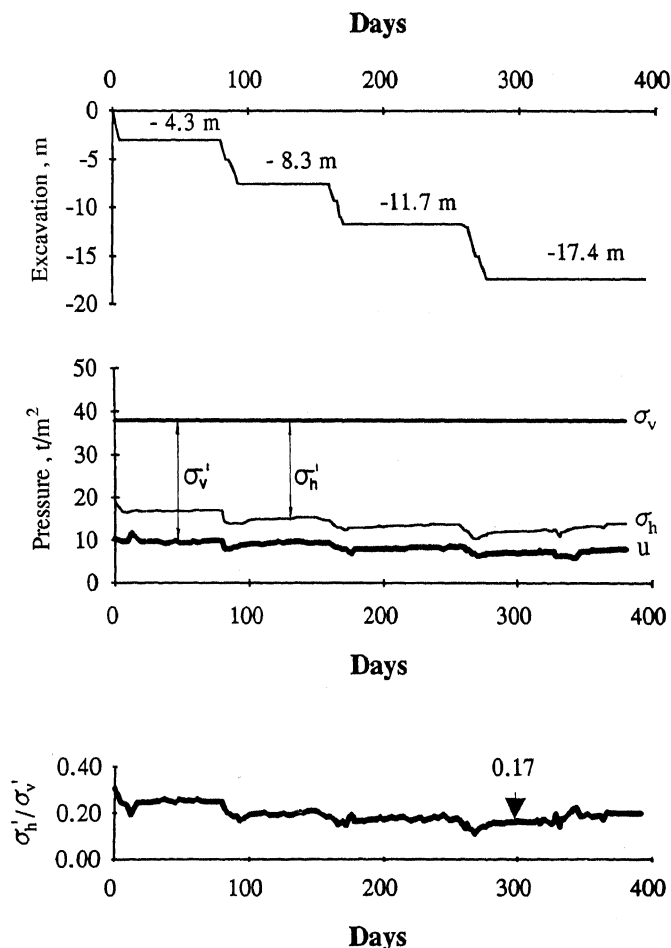
Figure 6 Active Pressures at a Depth of 20m
