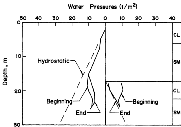
Figure 3 Distribution of Total and Water Pressures
