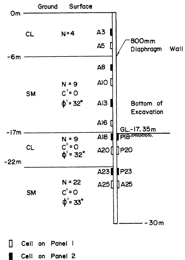
Figure 1 Soil Profile and Depths of Pressure Cells
