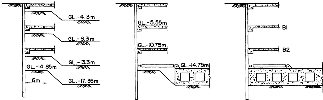
Figure 2 Sequence of Excavation
