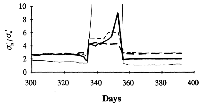
Figure 11 Results for All Cells on the Passive Side
