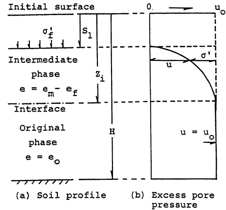
Fig.3 Soil profile and distribution of excess pore pressure
