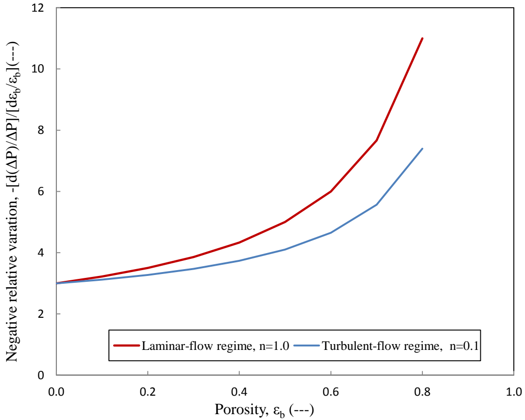
Figure 2.5. Effect of Void Fraction (Porosity) on the Pressure Drop in the Laminar and Turbulent Flow Regimes
