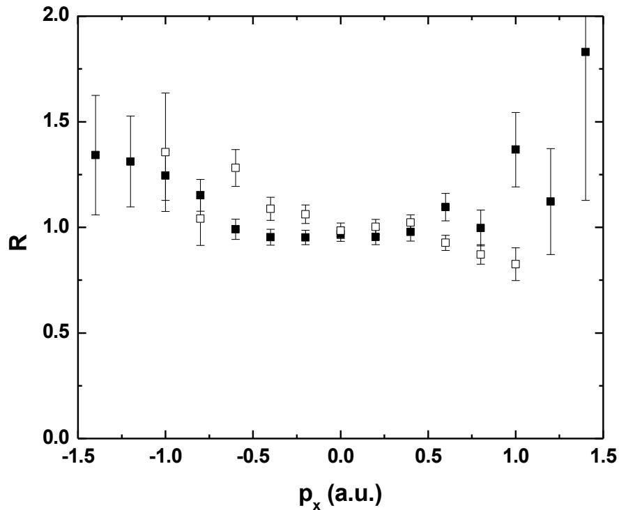
Figure 5: Ratio between the DDCS of Fig. 2 for large and small slit distances for the electrons (open symbols) and recoil ions (closed symbols).
