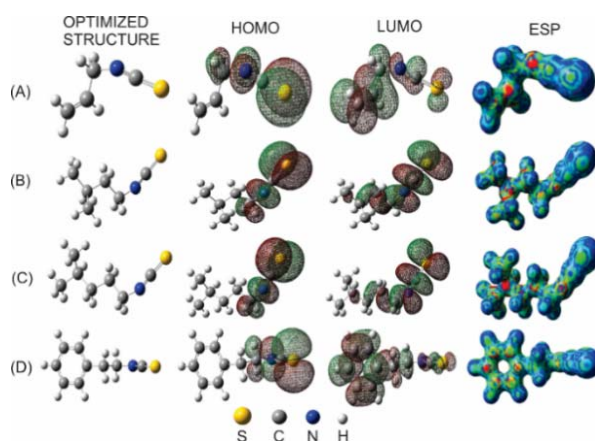
Figure 2. Optimized structures, HOMO, LUMO and electrostatic potential (ESP) structures of (A) 3ITCP, (B) 1ITC-3MB, (C) 1ITC-4MP, (D) 2ITC-EB. (ESP are displayed at an isovalue of 0.1 and mapped in range from 0.085 to 0.1)
