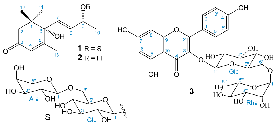
Figure 1. Structure of compounds 1 – 3.
