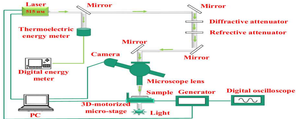
Figure 1. The schematic femtosecond laser pulses for fabrication microholes in thin metallic film.
