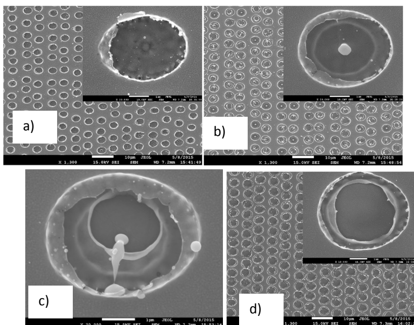
Figure 3. Scanning electron microscopy (SEM) image of the diffraction grating with diameter d \approx (a) 2, (b, c) 3, (d) 4 \mu\text{m} and period p \approx 6 \mu\text{m} of microhole arrays in the 150 nm thick silver film formed by strongly focused ultrashort laser pulses with the energy E \approx (a) 160, (b, c) 176, (d) 220 nJ in the single pulse ablation regime. (c) Magnified images of the microhole with diameter d \approx 3 \mu\text{m} with the nanojet. Scale bar: 10 \mu\text{m} .
