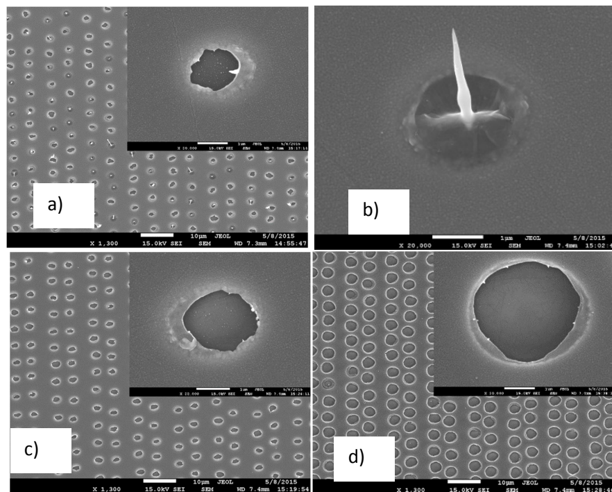
Figure 2. Scanning electron microscopy (SEM) image of the diffraction grating with diameter d \approx (a, b) 2, (c) 3, (d) 4 \mu\text{m} and period p \approx 6 \mu\text{m} of microhole arrays in the 100 nm thick silver film formed by strongly focused ultrashort laser pulses with the energy E \approx (a, b) 72, (c) 80, (c) 104 nJ in the single pulse ablation regime. (b) Magnified images of the microhole with diameter d \approx 2 \mu\text{m} with the nanojet. Scale bar: 10 \mu\text{m} .
