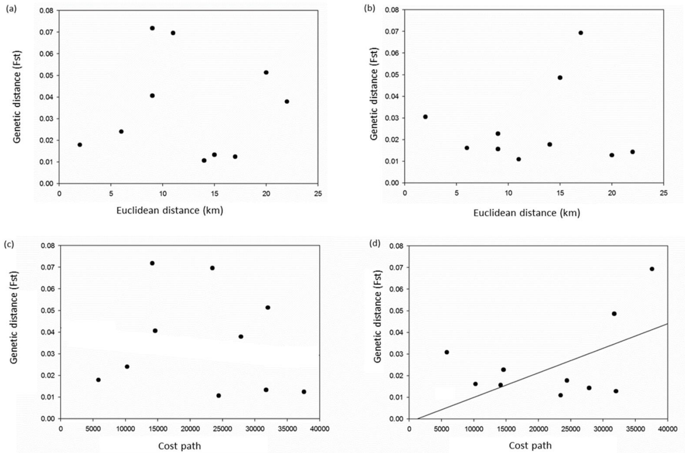
Figure 3.2. Associations between Euclidean distance and least cost path with genetic distance.
