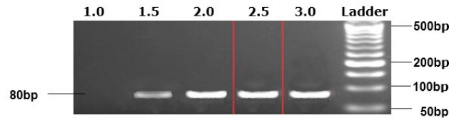
Figure 4. Optimizing MgCl 2 concentration in the range [1.0, 3.0] mM on gel electrophoresis.
