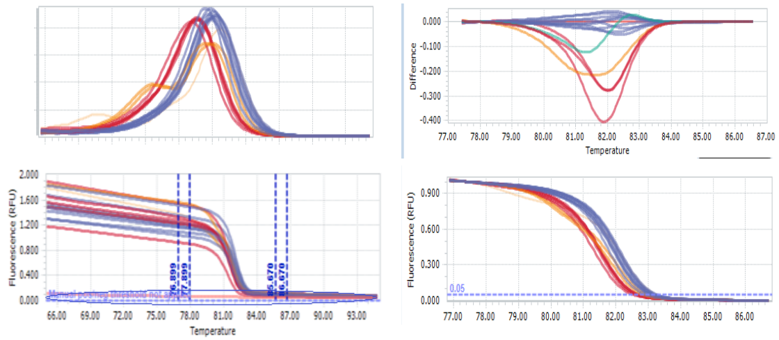
Figure 6. Massively genotyping for 50 samples. Blue, Red and Orange curves represent for melting curve of genotype YG, YA, GA, respectively.
