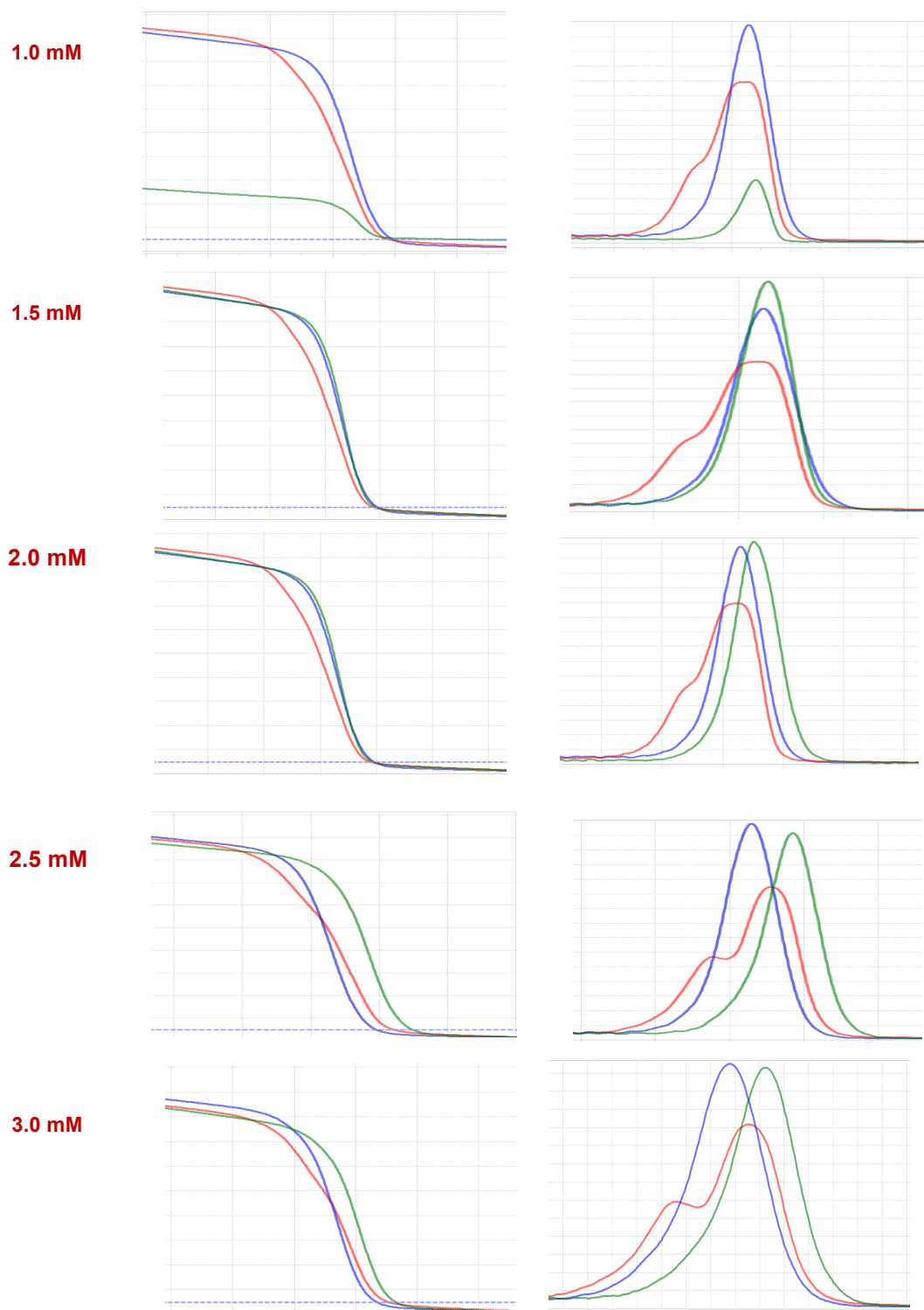
Figure 3. Affecting of MgCl 2 concentration on discrimination of 3 genotypes in Normalized Melting Curves and Normalized Melting Peaks. Green, Blue and Red curves/peaks represent for melting curves/peaks of genotype YG, YA, GA, respectively.
