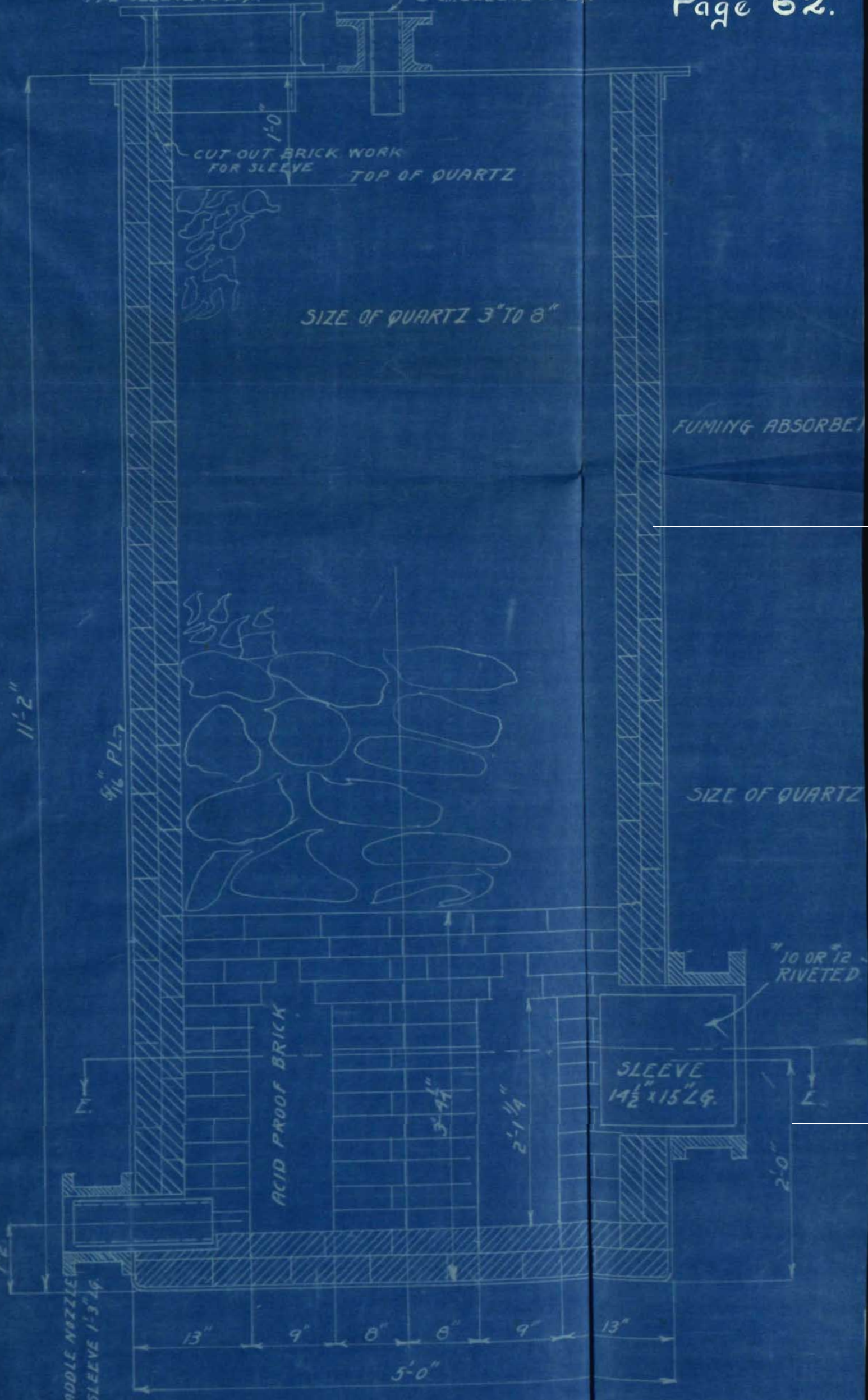
FUMING ABSORBER SECTION C.C. SCALE 1"=1'0"
