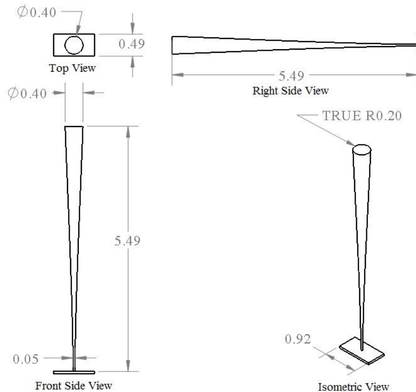
Figure 31: Detailed dimension of Vortex Bladeless Wind Generator
