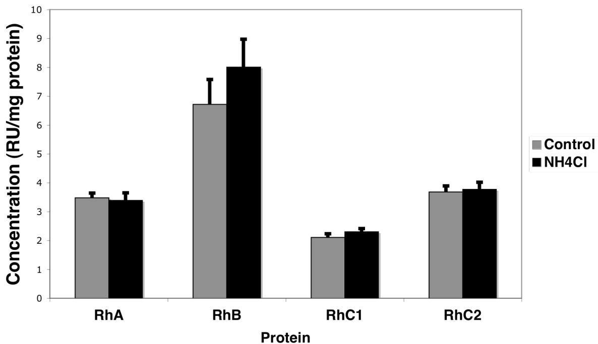
Figure 15: Acute relative \text{NH}_4\text{Cl} protein expression. Graph showing the relative expression of sculpin RhAg, RhBg, RhC1g, and RhC2g protein in gill after acute ammonia stress of \text{NH}_4\text{Cl} treatments, and water control, \bar{x} \pm \text{SE} N=6 for each group. RhAg p=0.88 , RhBg p=0.63 , RhC1g p=0.57 , RhC2g p=0.88 .
