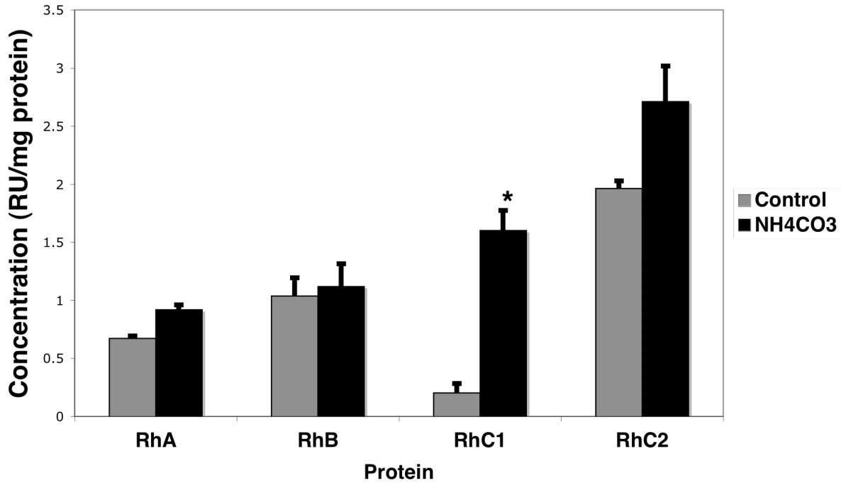
Figure 17: Chronic relative \text{NH}_4\text{HCO}_3 protein expression. Graph showing the expression of sculpin RhAg, RhBg, RhC1g, and RhC2g protein in gill after chronic ammonia stress of \text{NH}_4\text{HCO}_3 treatment and water control, \bar{x} \pm \text{SE} N=3 for each group. RhAg p=0.06 , RhBg p=0.88 , p=0.02^* , RhC2g p=0.29 .
