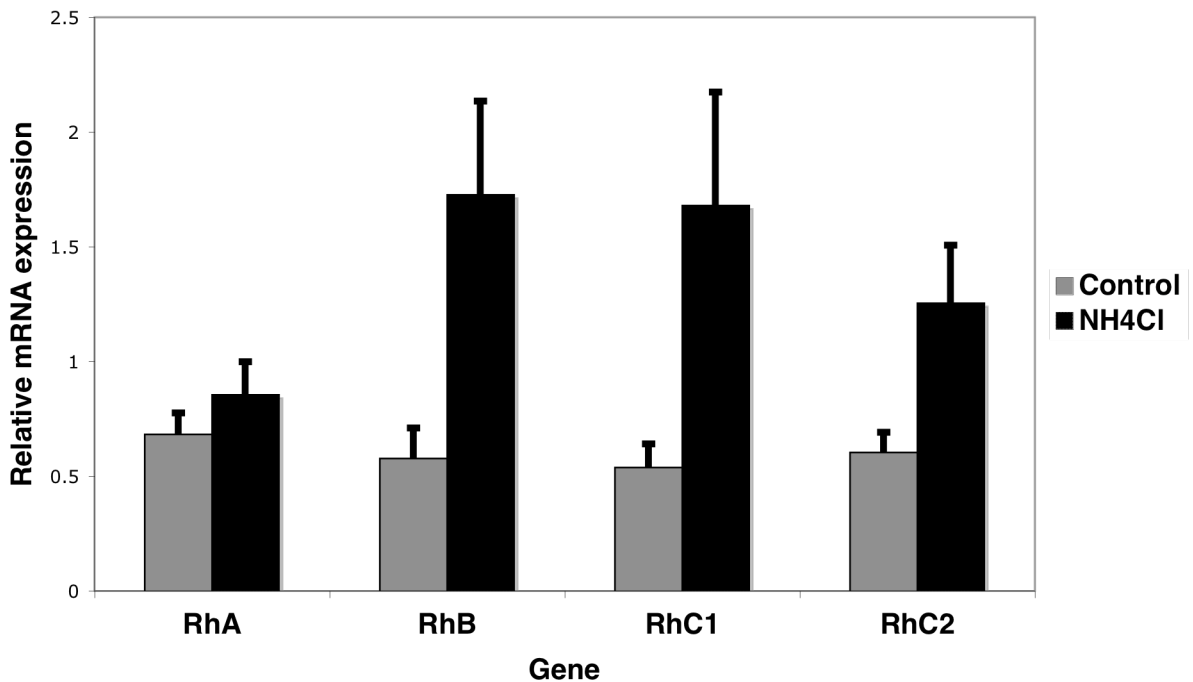
Figure 8: Acute relative \text{NH}_4\text{Cl} mRNA expression. Graph showing relative expression of sculpin RhAg, RhBg, RhC1g, and RhC2g mRNA compared to Ubc internal control in the gill after acute ammonia stress of \text{NH}_4\text{Cl} treatments, and water control, x \pm \text{SE} N=6 for each group. RhAg p=0.62 , RhBg p=0.2 , RhC1g p=0.28 , RhC2g p=0.25 .
