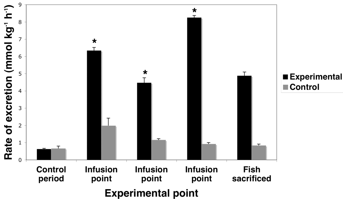
Figure 6: Rate of ammonia efflux. Experimental NH 4 HCO 3 treatment and water control, \bar{x} \pm SE N=3 for each group. Control rates compared to pre-infusion control (time 0): P=0.167, p=0.313, 0.604, and p=0.447 respectively for time 2, 4, 6, and 8. Experimental rates compared to pre-infusion control (time 0): p=0.004*, p=0.023*, p=0.0009*, and p=0.013 respectively for time 2, 4, 6, and 8 utilizing Bonferroni adjusted \alpha rates.
