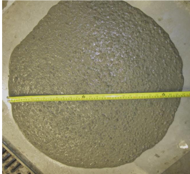
Figure 5.10 Slump flow.
