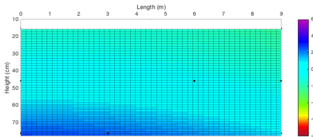
Figure 6.27 Compressive strength results in absolute values for beam 7 (Avg. f'_c = 47.7 MPa).
