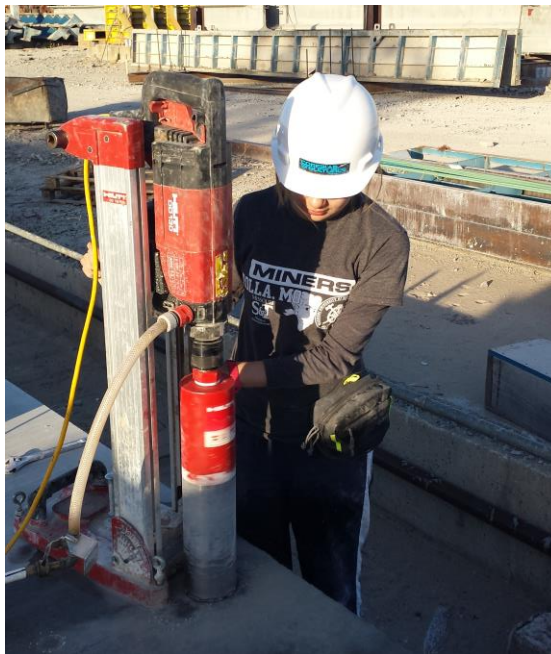
Figure 5.18 Extracting cores from a beam.
