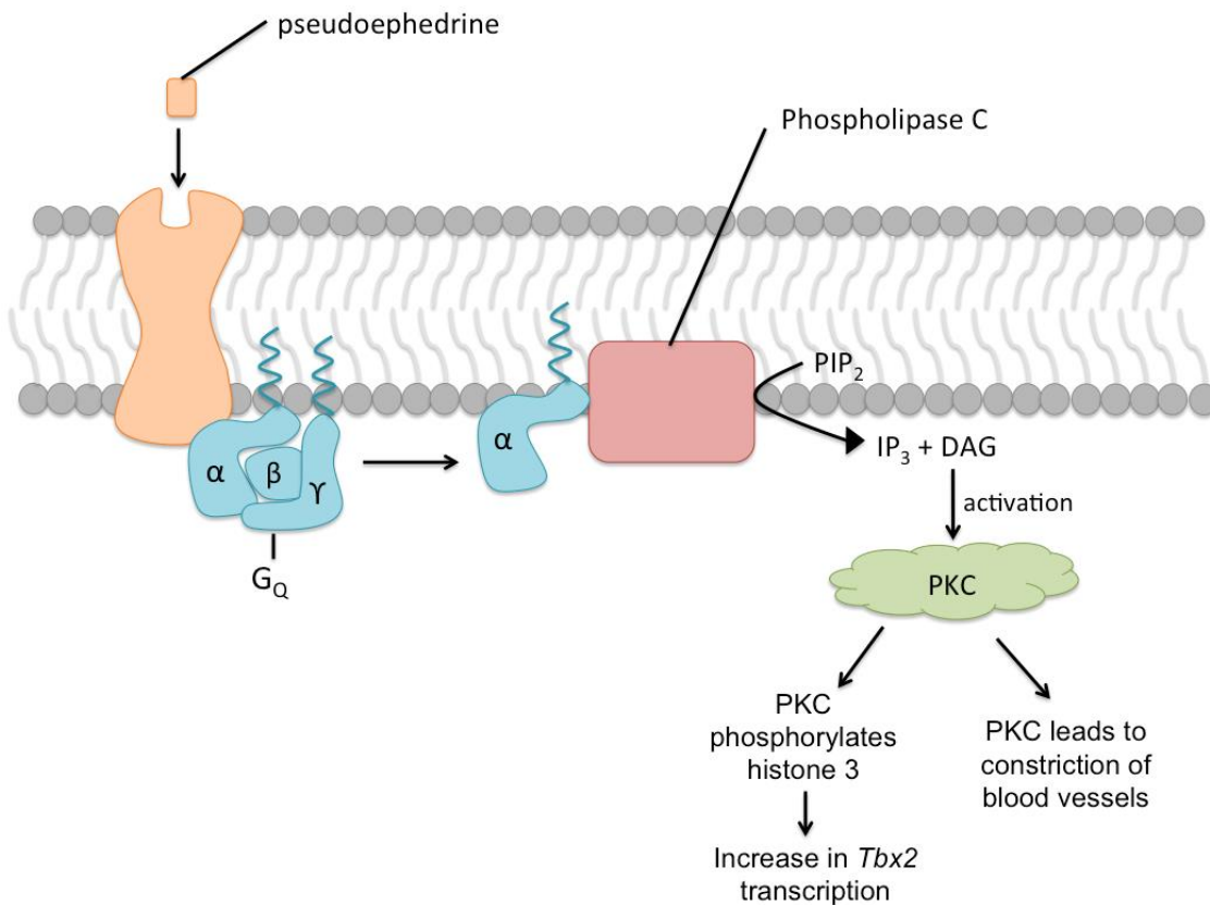
Figure 2.2. Mechanism of PKC activation by pseudoephedrine via the G q pathway.
