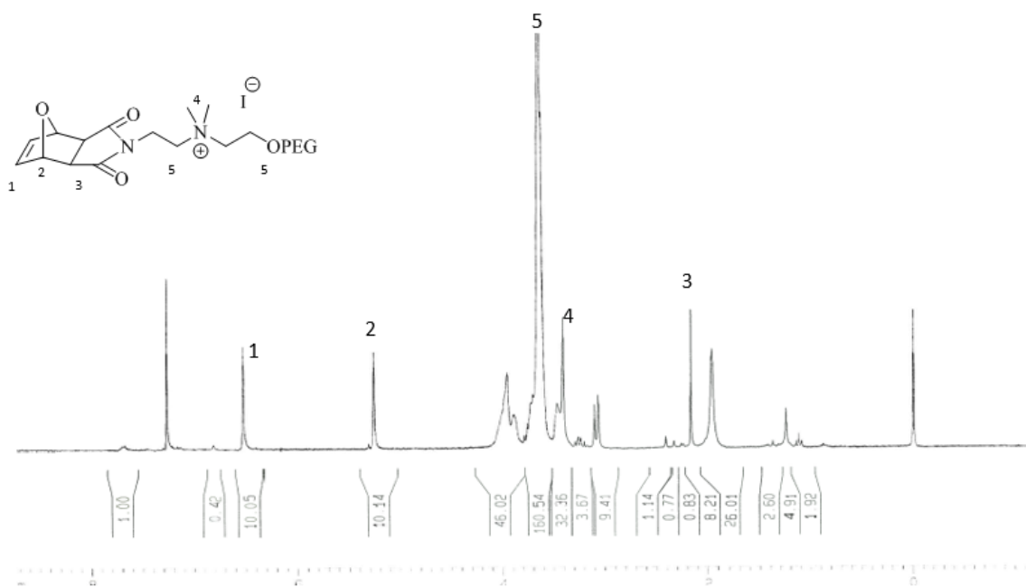
Figure 2: ^1\text{H} NMR of cationic PEG-monomer, 250 MHz, \text{CDCl}_3
