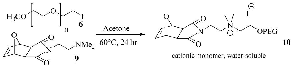
Scheme 4. Synthesis of Cationic, PEG-containing Exo-7-oxanorbornene Derivative
