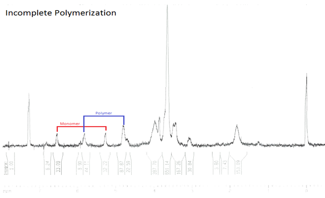
Figure 3: ^1\text{H} NMR spectrum ( \text{CDCl}_3 , 250 MHz) of the polymerization mixture after addition of terminating agent and removal of solvent.
