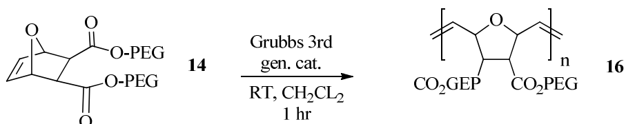
Scheme 7. Synthesis of ROMP homopolymer bearing PEG
