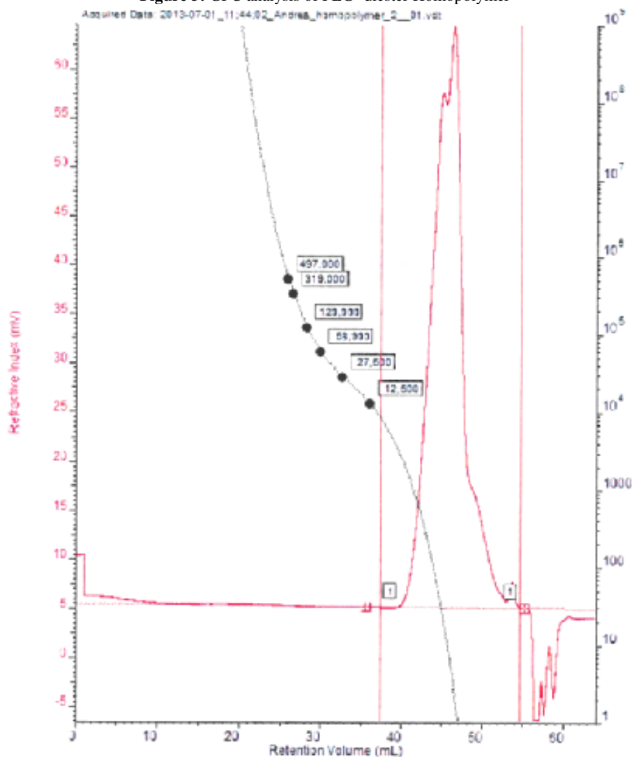
Figure 5: GPC analysis of PEG- diester Homopolymer
