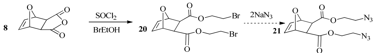
Scheme 10. Synthesis of Neutrally Charged Bromo diester monomer
