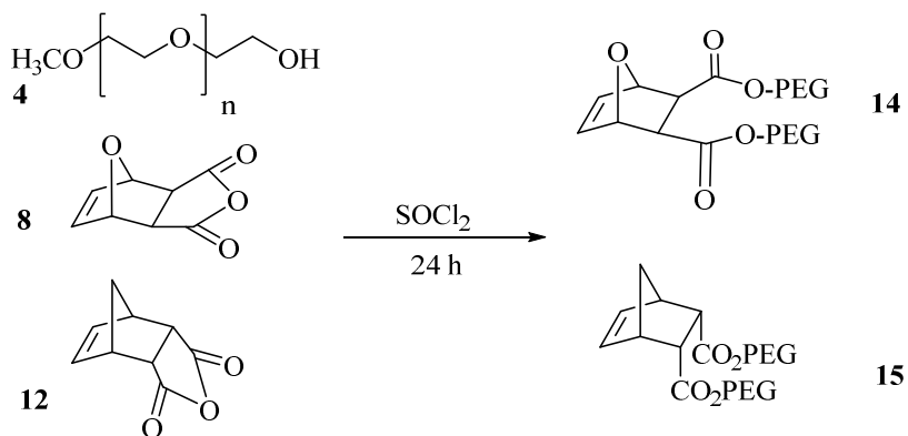
Scheme 6. Direct esterification of (7-oxa)-norbornene precursors resulting in neutrally charged diester monomers
