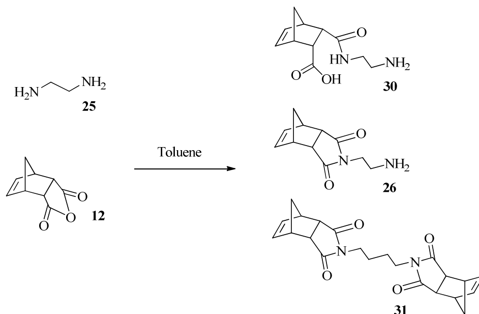
Scheme 13. Amination of Endo-norbornene anhydride through four different conditions
