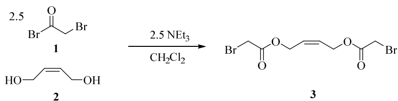
Scheme 1. Synthesis of Chain Transfer Agent for Termination of ROMP
