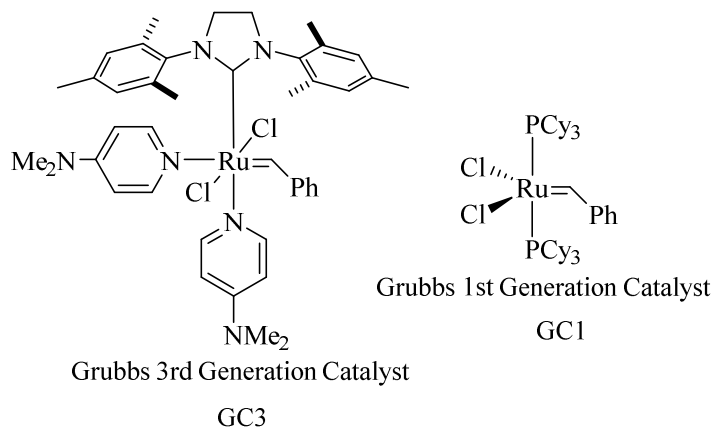
Figure 1: Ruthenium based catalysts used for controlled polymerization of Pegylated ROM monomers
