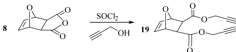
Scheme 9. Synthesis of Neutrally Charged alkyne diester monomer
