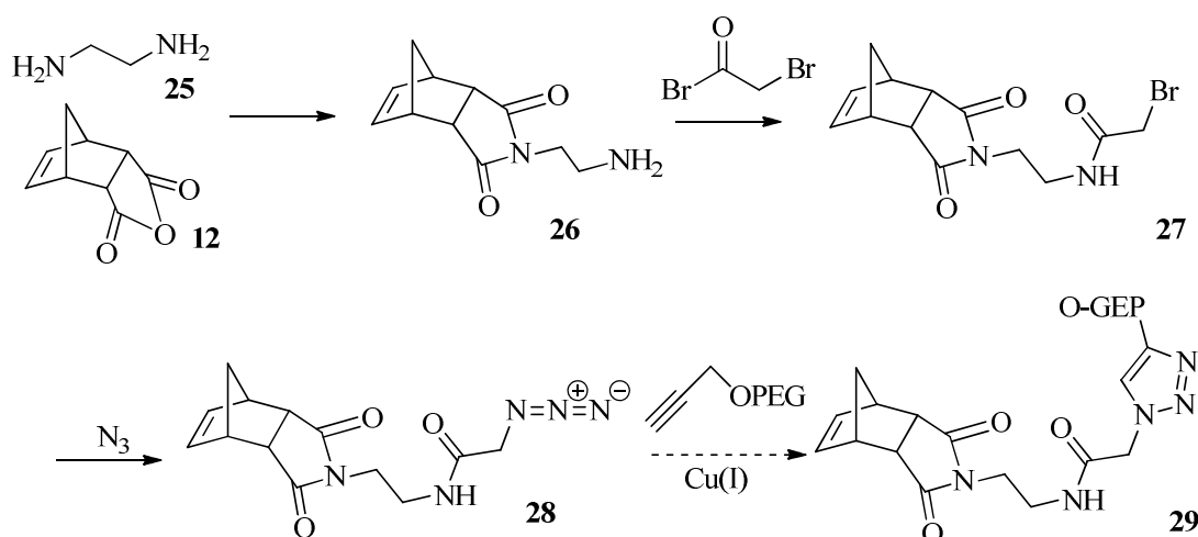
Scheme 12. Proposed synthesis of endo-norbornene pegylated triazole monomer
