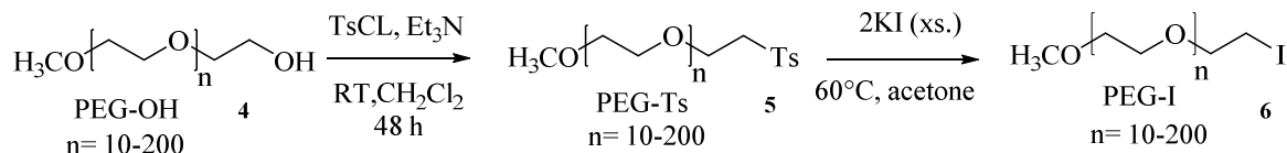
Scheme 2. Synthesis of Polyethylene Glycol Iodide using a series of nucleophilic substitution reactions.
