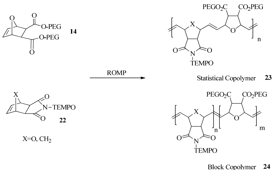
Scheme 11. Planned Synthesis of ROMP copolymers bearing PEG and TEMPO groups
