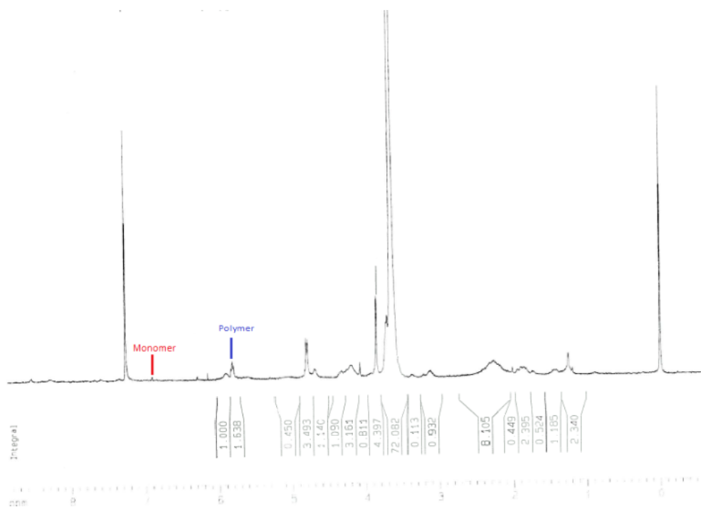
Figure 5: ^1\text{H} NMR spectrum ( \text{CDCl}_3 , 250 MHz) of the ROMP Polymerization of 7-oxa-norbornene diester monomer
