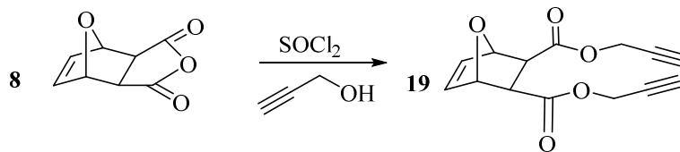
Scheme 9. Synthesis of Neutrally Charged alkyne diester monomer
