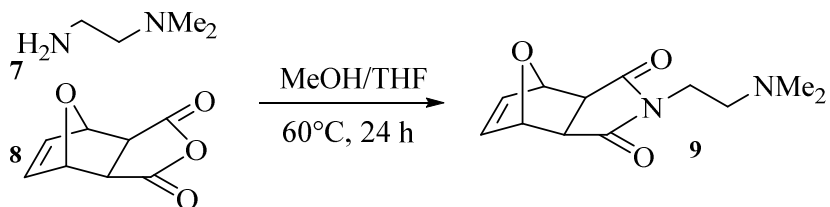
Scheme 3. Synthesis of Dimethylamino Imide monomer from Carboxylic Anhydride
