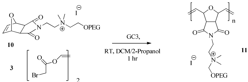
Scheme 5. ROMPolymerization of cationic-monomer, 5% catalyst loading with 3rd generation catalyst
