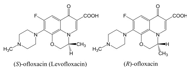
Fig. 1: Structures of levofloxacin and ofloxacin
