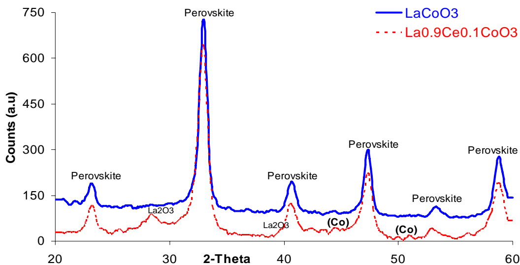
Figure 4: XRD patterns of La 1-x Ce x CoO 3 reduced at 400°C under hydrogen atmosphere for 90 min
