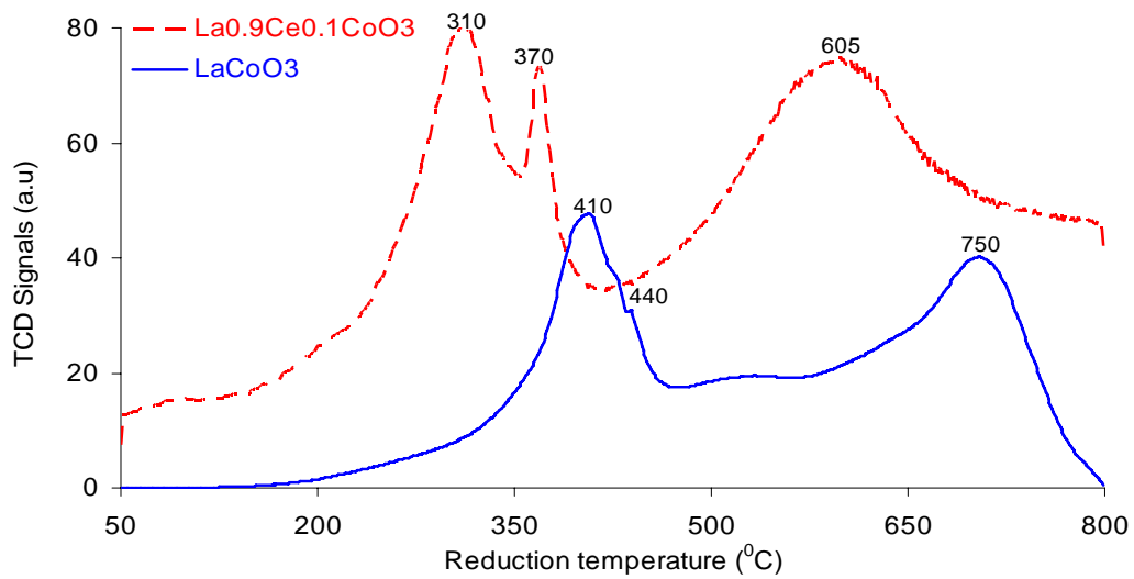
Figure 3: H 2 -TPR of the two ground perovskites
