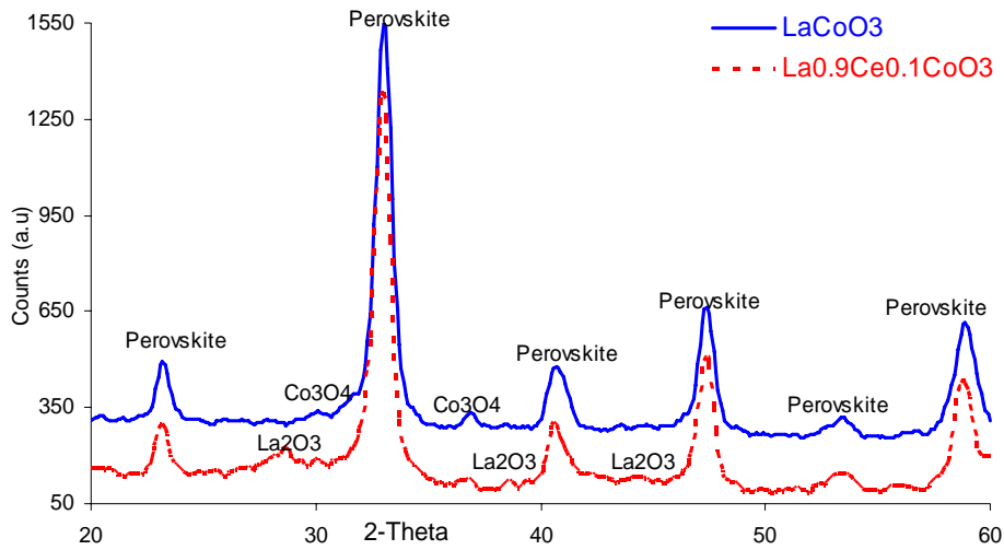
Figure 2: X-ray diffraction patterns of La 1-x Ce x CoO 3
