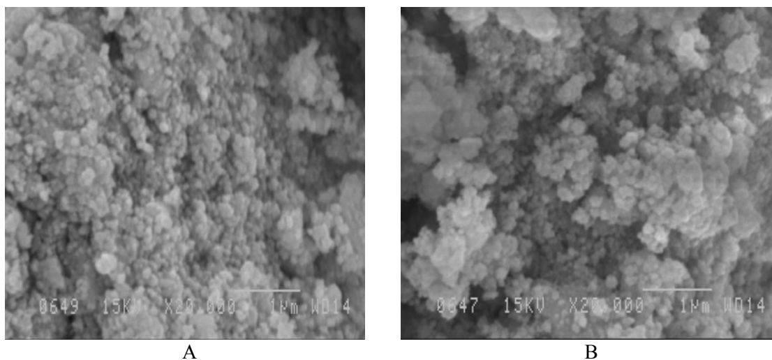
Figure 1: SEM photographs of LaCoO_3 (A) and La_{0.9}Ce_{0.1}CoO_3 (B) nanocrystalline perovskites after calcined at 250^\circ C
