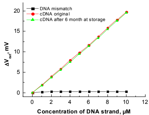
Figure 3: The lifetime of the DNA sensor
