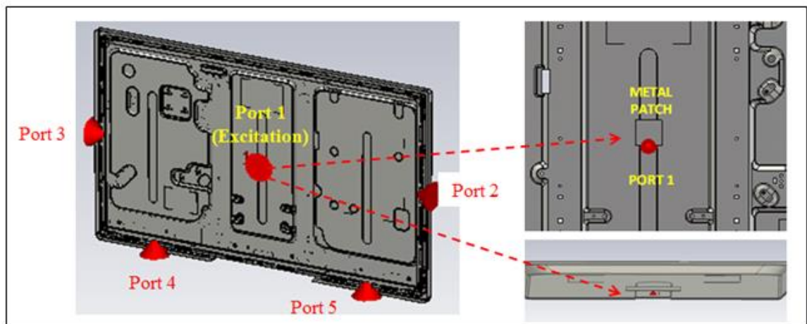
Figure 4.14. Simulation model
