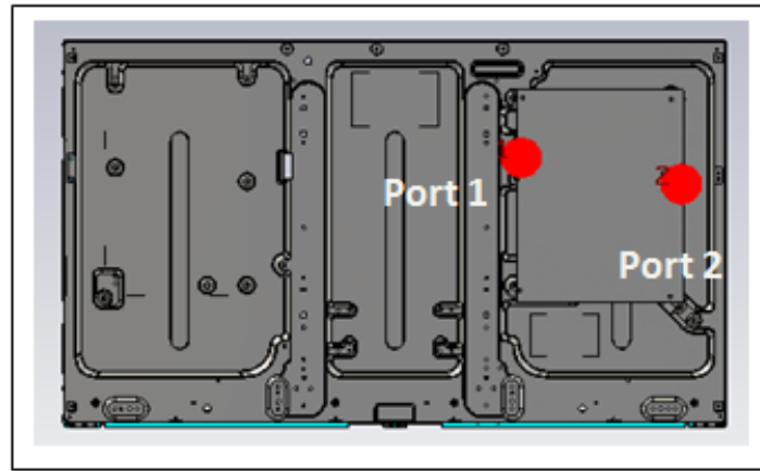
Figure 4.28. Simulation model
