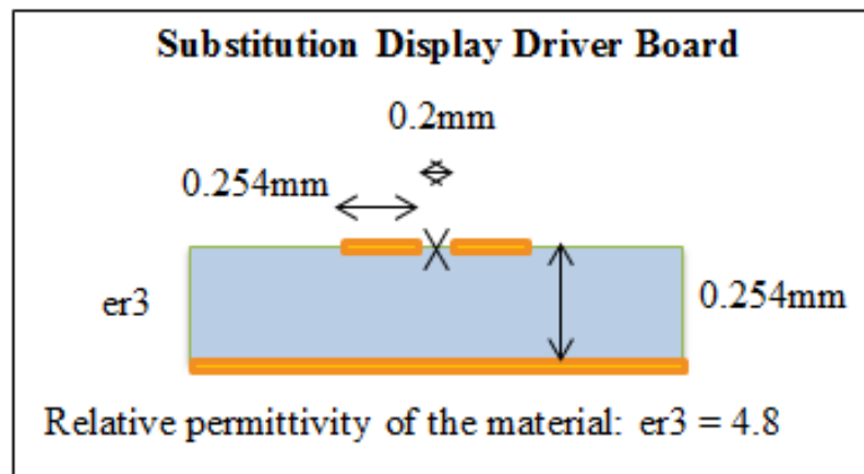
Figure 4.48. Substitution display driver board cross-section
