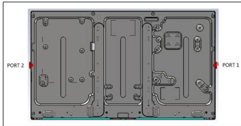
Figure 4.5. Simulation Model
