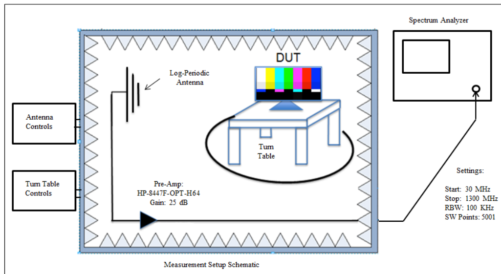
Figure 2.4. Measurement setup
