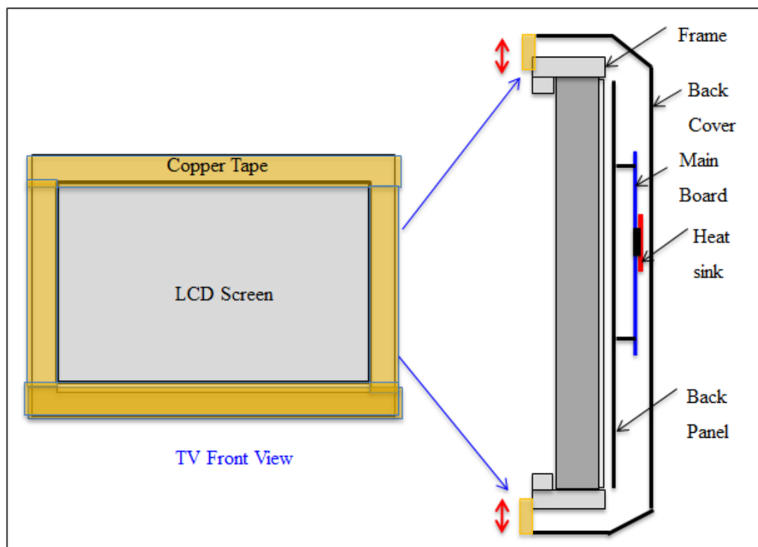
Figure 2.14. Diagram showing the front gaps covered with copper tapper tape
