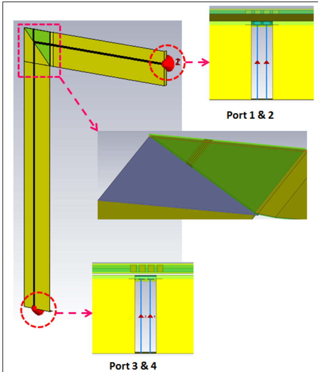
Figure 4.35. Simulation model
