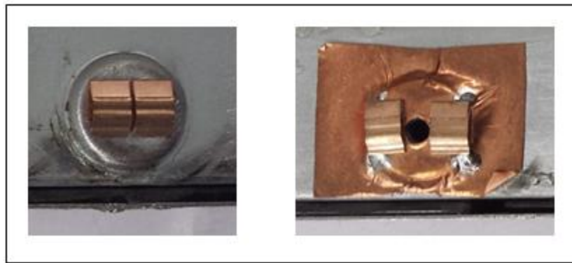
Figure 4.2. Gaskets connections on back panel for better contact to back cover
