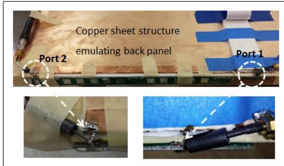
Figure 4.50. Measurement setup
