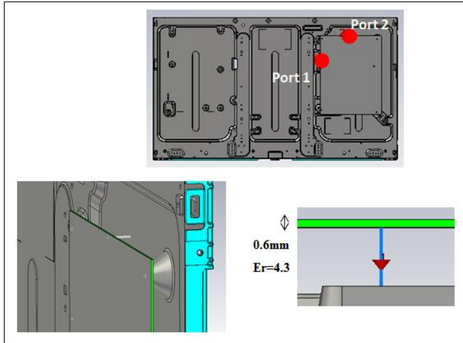
Figure 4.24. Simulation model
