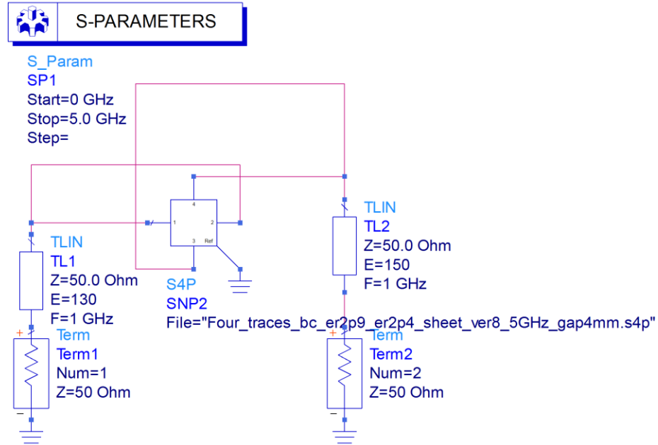
Figure 4.356. ADS model
