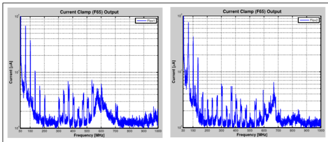
Figure 3.9. Common-mode current on Flex 2
