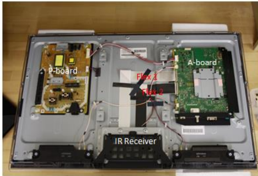
Figure 3.2. Inside of TV1
