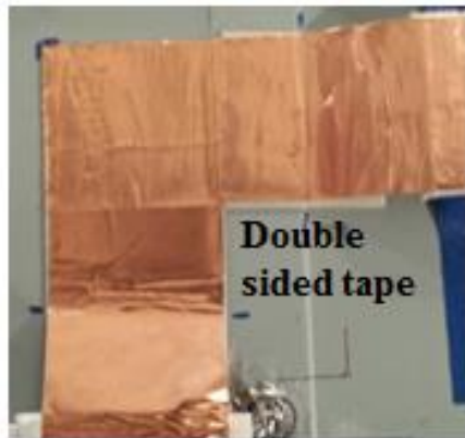
Figure 5.7. Flex cable bend region 0.8 mm above the back panel
